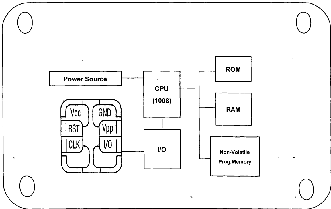
FIGURE 1D. Exposed view of an exemplary multifunction removable cover embodiment
