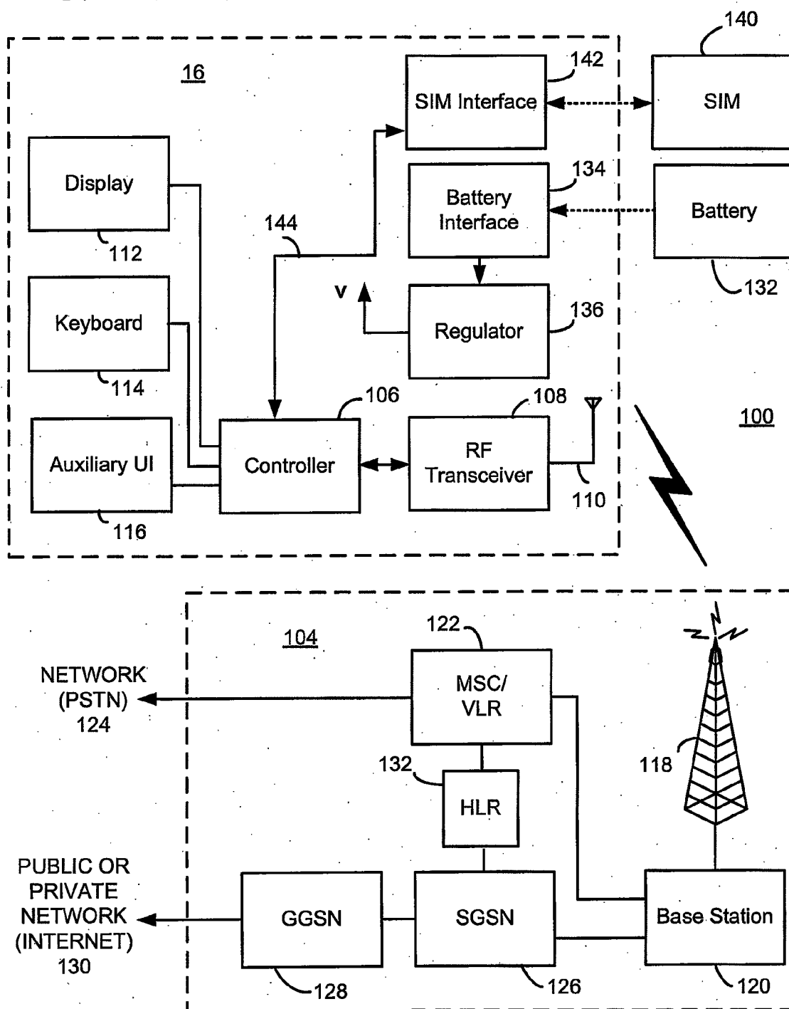
FIG. 5: GPRS Device
