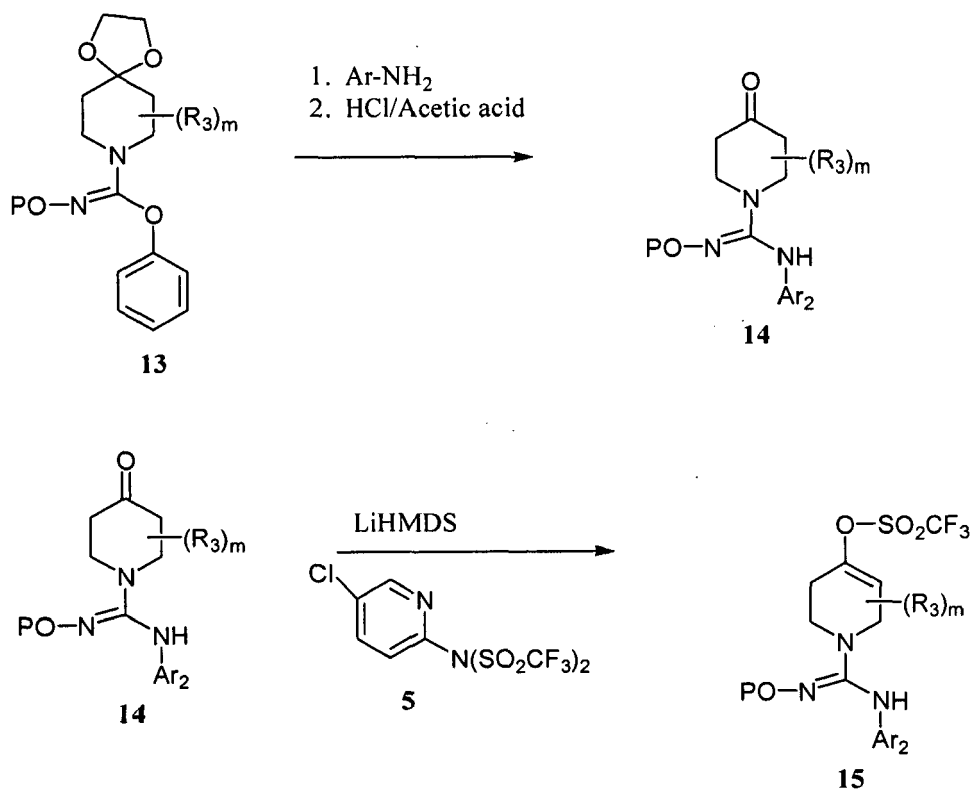
Scheme 6
