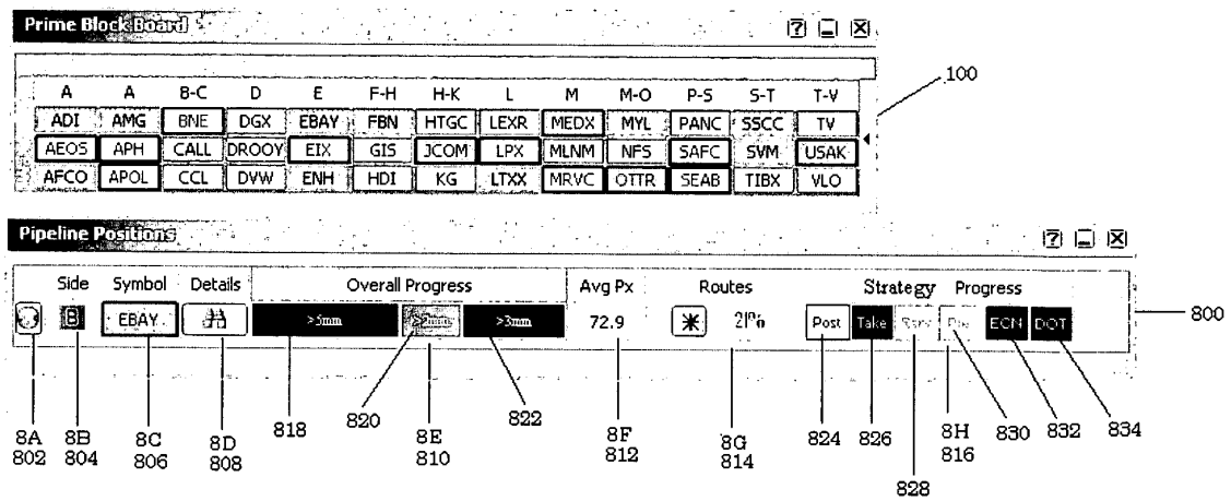
Figure 8: Positions Window
