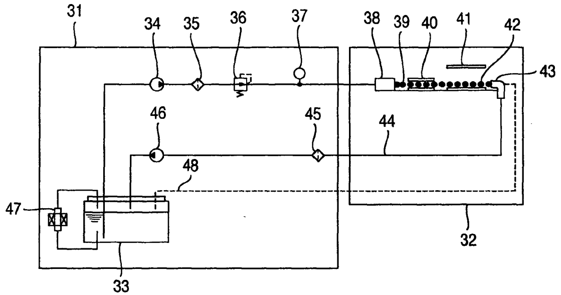
FIG.7 PRIOR ART
