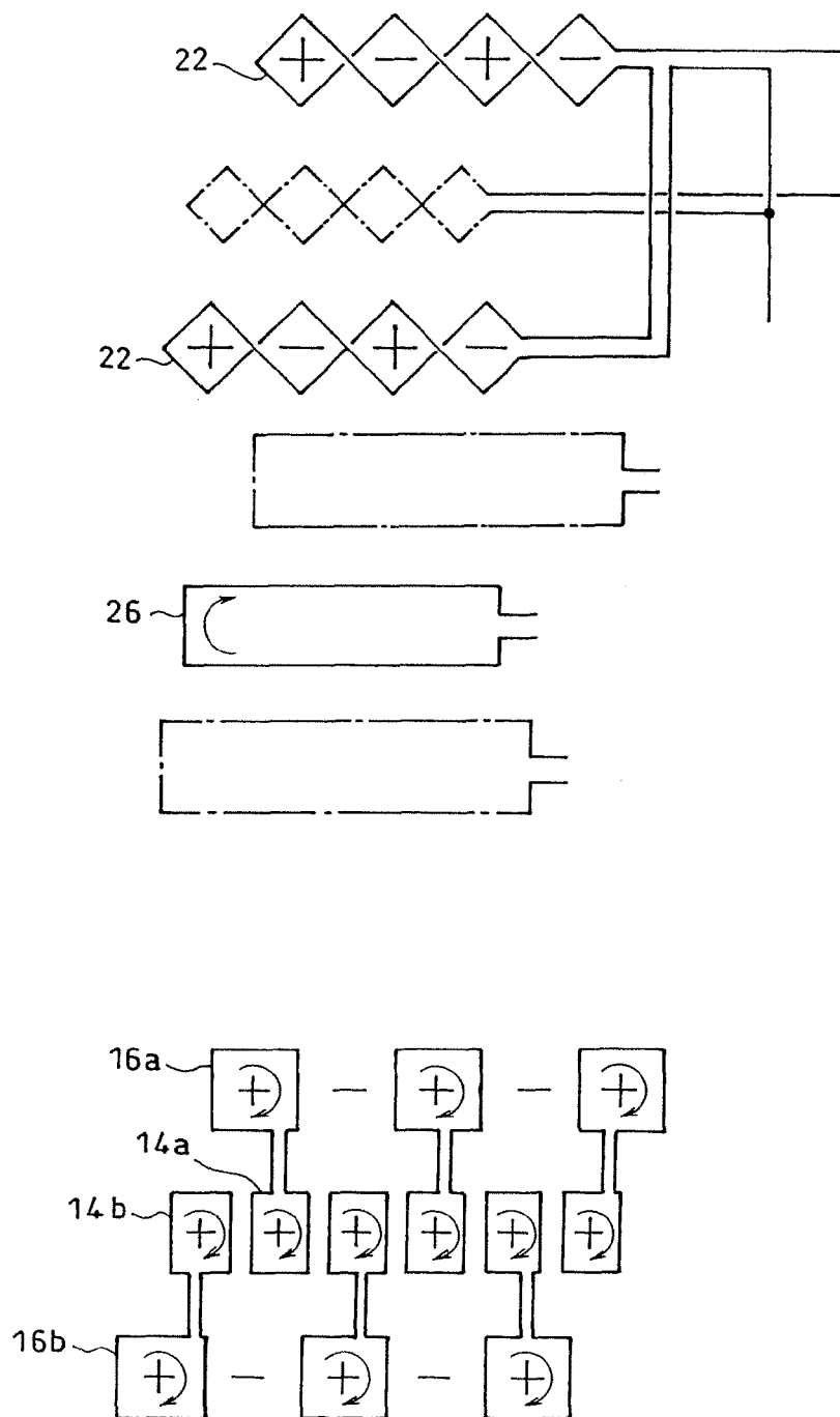
Fig. 3 PRIOR ART
