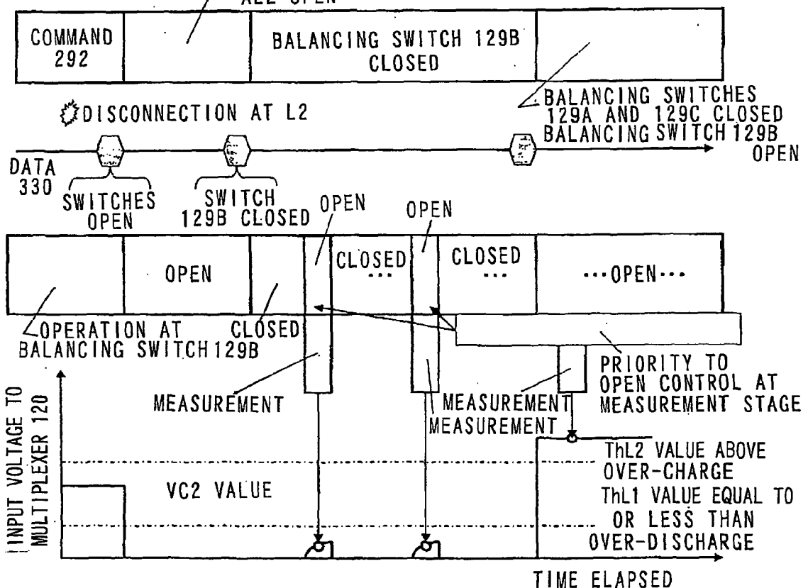
FIG.29 BALANCING SWITCHES 129 ALL OPEN
