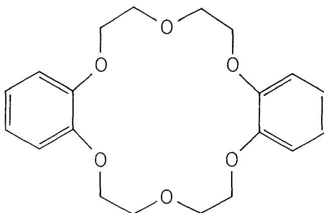
DIBENZOYL-18-CROWN-6
