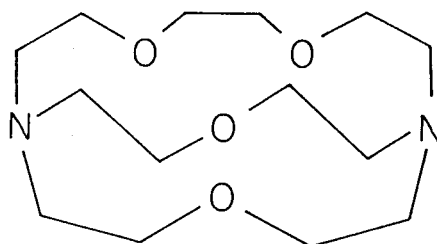
CRYPTAND [2.1.1]
