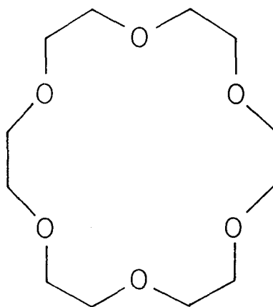
18-CROWN-6
