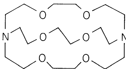
CRYPTAND [2.2.2]
