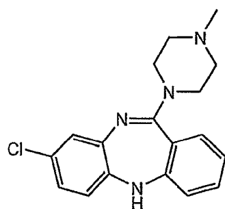
Clozapine
