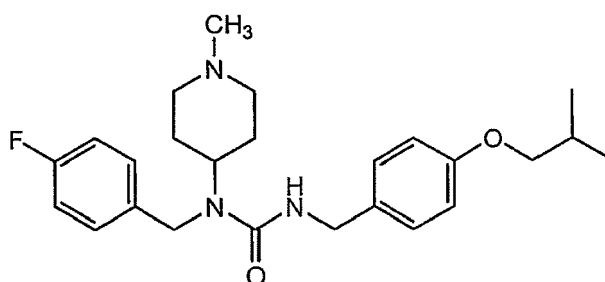
(XIII)
