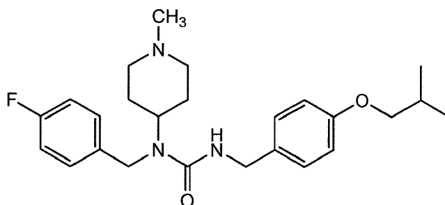
(XIII)
