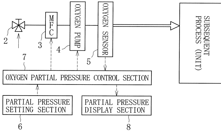
FIG. 10 (Prior Art)
