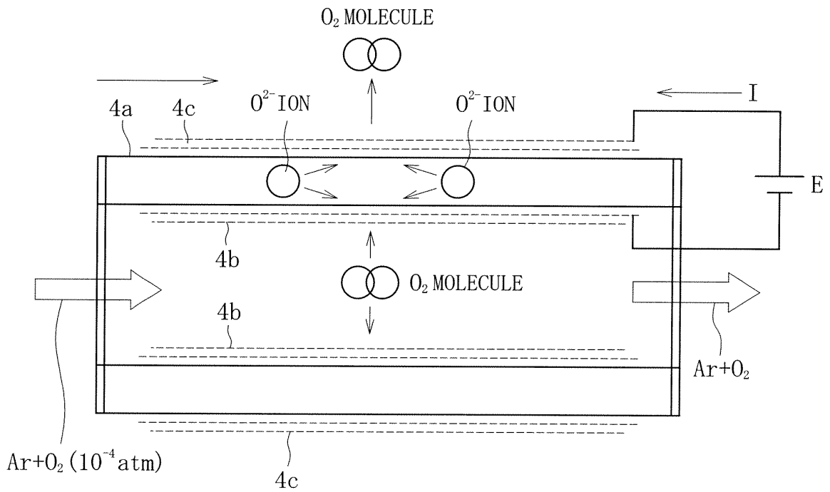
FIG. 10 (Prior Art)
