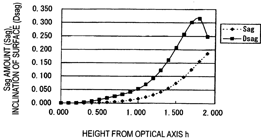
EXAMPLE 9 : SURFACE FORM OF THIRD LENS G3 ON OBJECT SIDE
