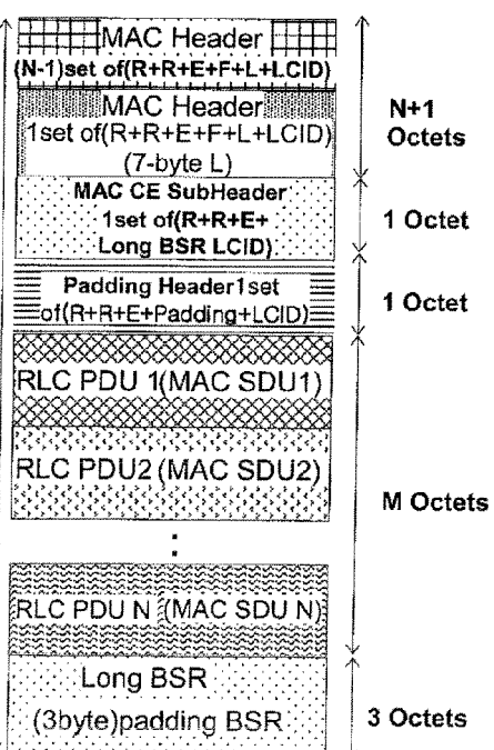
(c) case 3, 7-bit L field for the last MAC SDU
