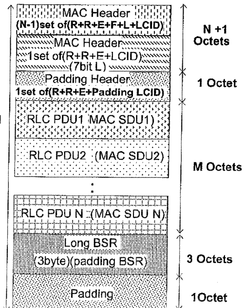
(c) case 3, implicit padding BSR
