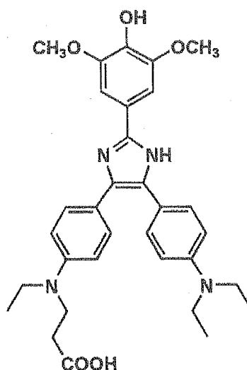
Compound 2
