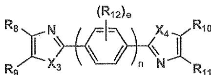
Formula [3]
