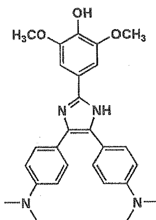
Compound 1
