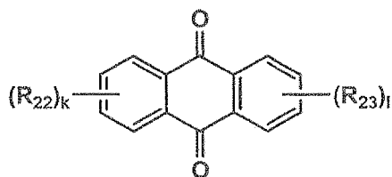
Formula [5]
