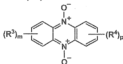
Formula (III)
