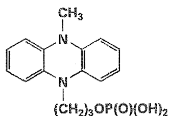
Compound (A)
