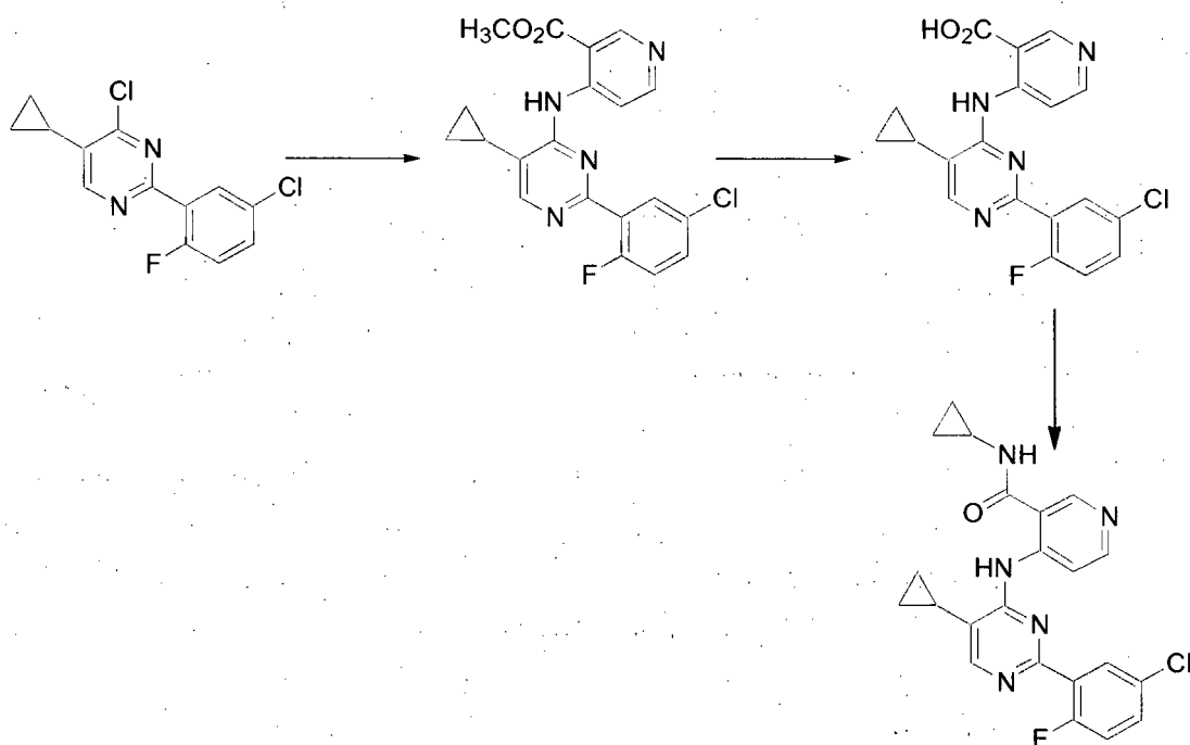
Scheme 8
