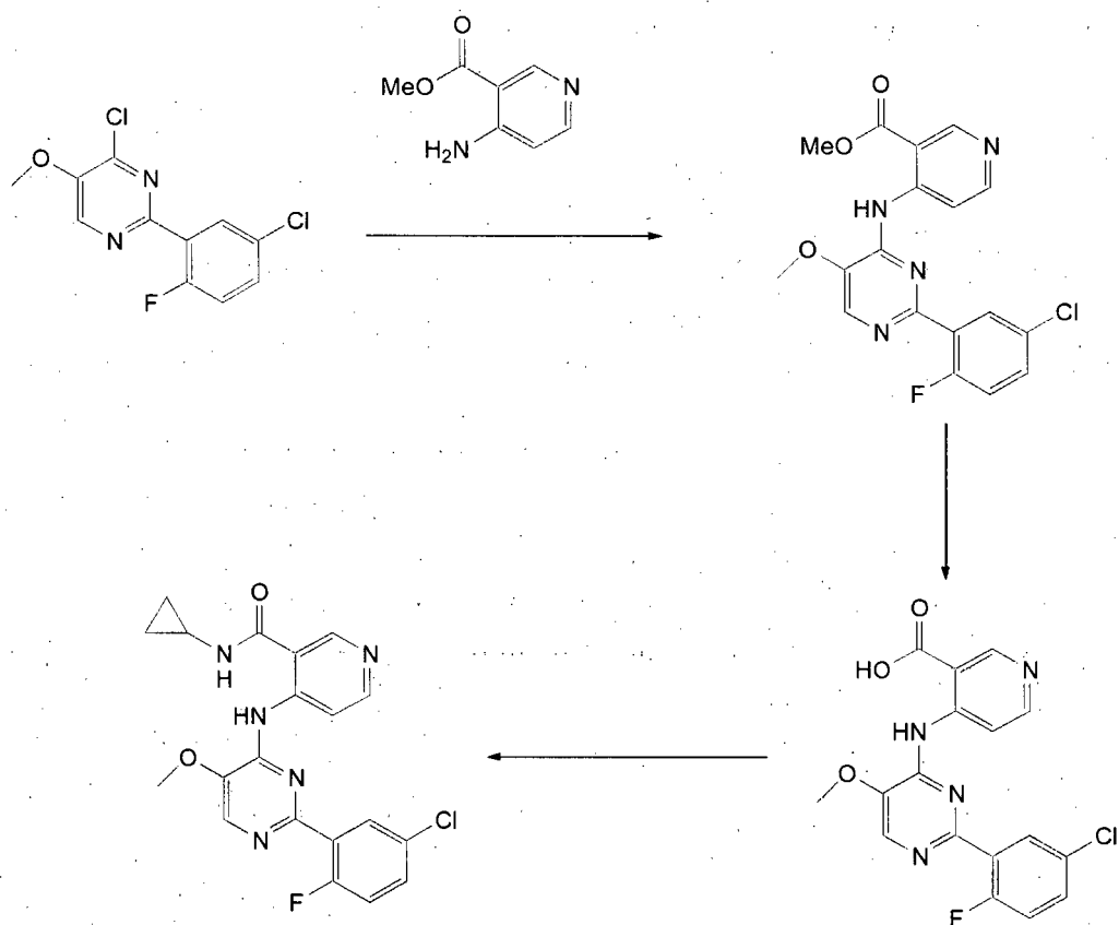
Scheme 6
