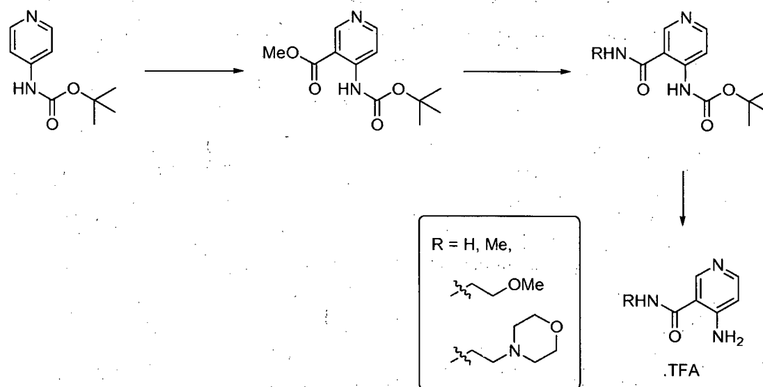
Scheme 5
