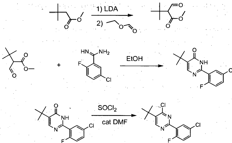
Scheme 12
