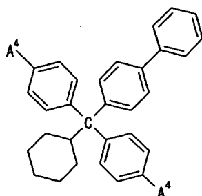
Compound No. 4
