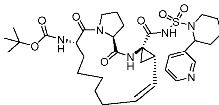
Compound 2222
