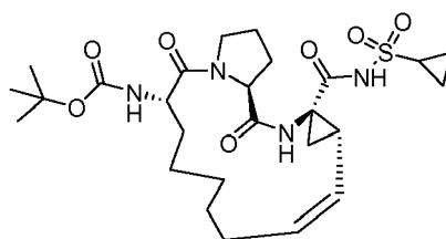
Compound 2137
