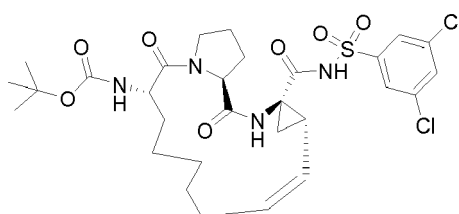
Compound 2108
