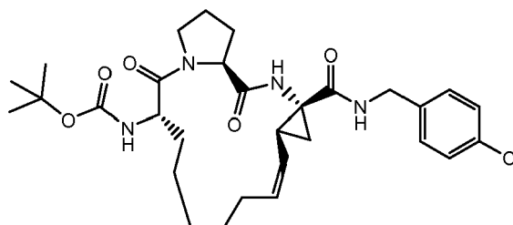
Compound 2308
