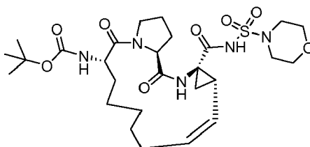
Compound 2204
