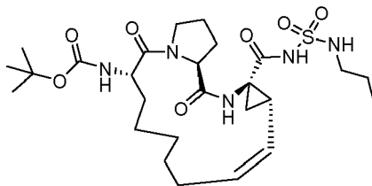
Compound 2217
