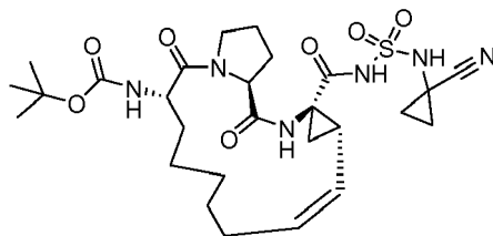
Compound 2212
