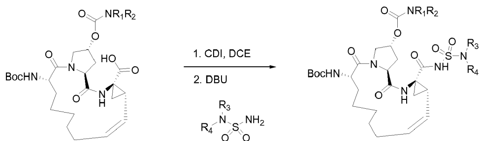
Scheme 3
