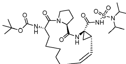
Compound 2209
