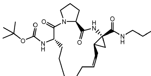
Compound 2319
