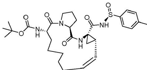
Compound 2402
