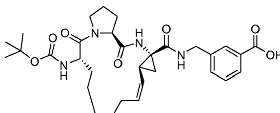
Compound 2310
