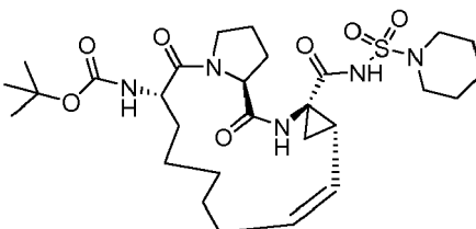
Compound 2219
