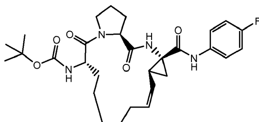
Compound 2304
