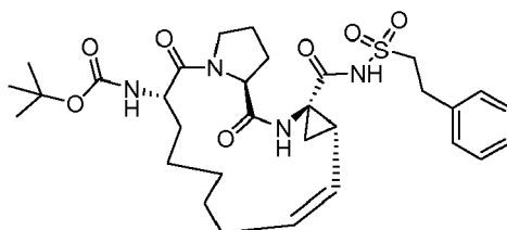
Compound 2127
