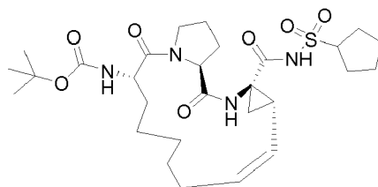
Compound 2120
