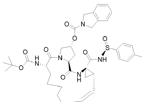
Compound 2602
