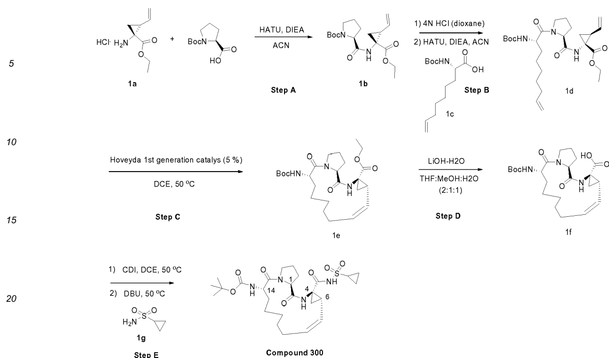
Scheme 4
