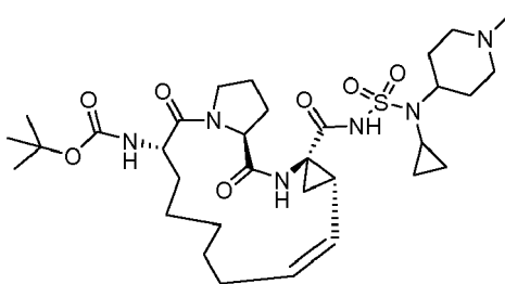
Compound 2211
