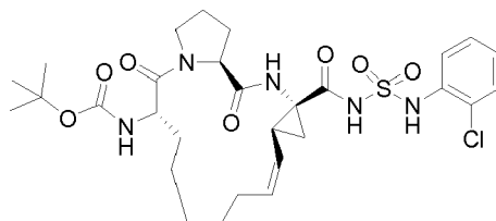
Compound 2233
