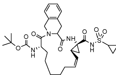
Compound 2009
