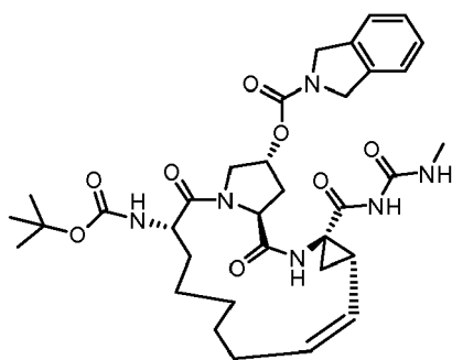
Compound 703
