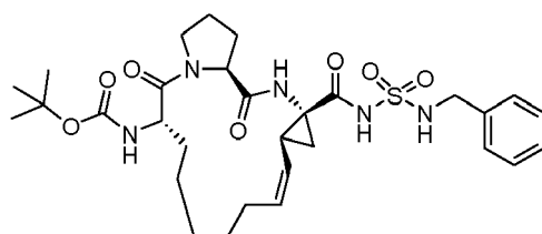
Compound 2232
