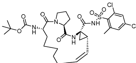
Compound 2123
