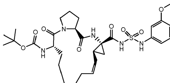
Compound 2240
