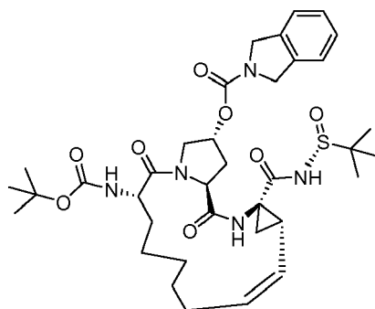
Compound 2604
