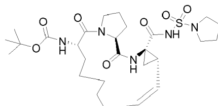
Compound 2207
