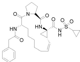
Compound 2144
