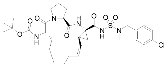
Compound 2230
