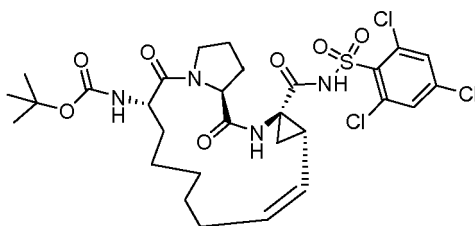
Compound 2115
