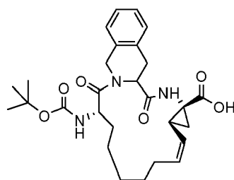
Compound 2001
