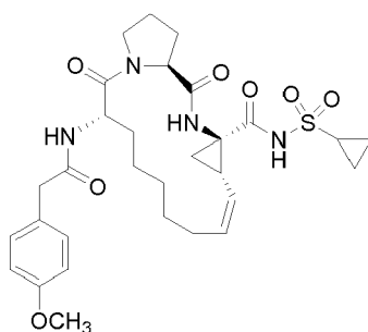
Compound 2138
