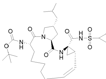
Compound 2147
