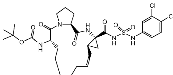
Compound 2234
