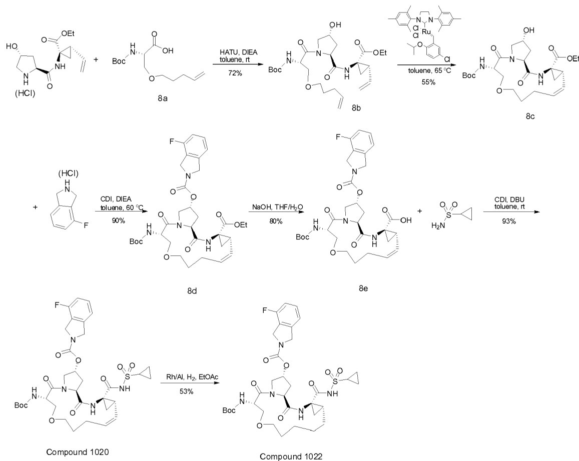
Scheme 8
