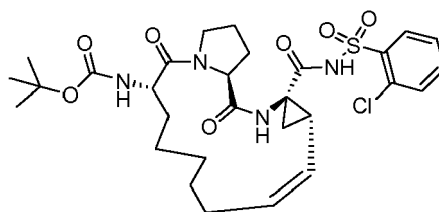
Compound 2109
