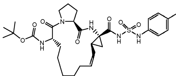
Compound 2243
