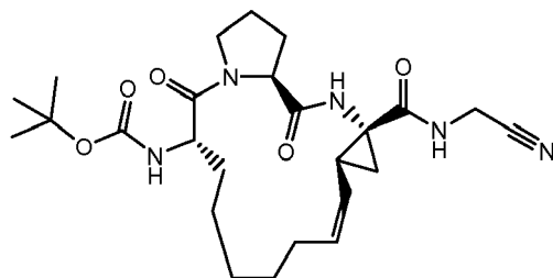
Compound 2322
