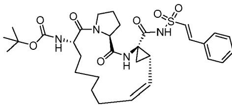
Compound 2125
