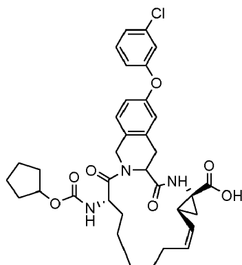
Compound 2002
