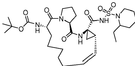
Compound 2220
