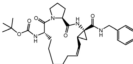
Compound 2307
