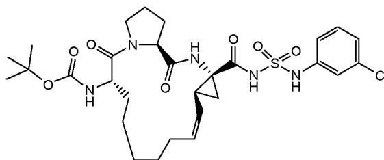
Compound 2239
