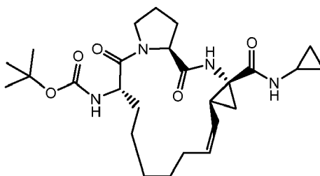
Compound 2318
