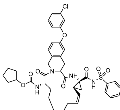
Compound 2004
