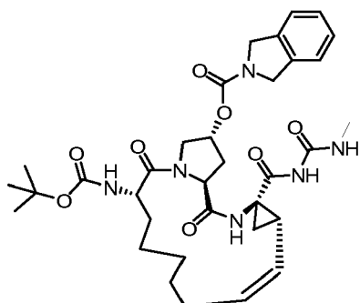
Compound 702
