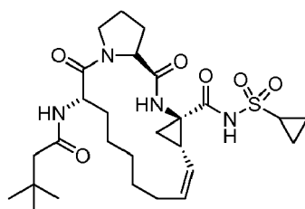
Compound 2141
