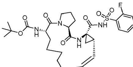
Compound 2124
