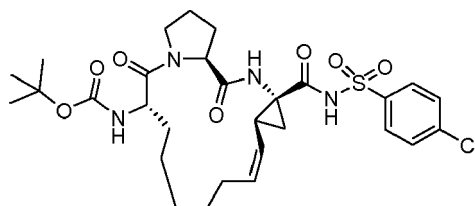
Compound 2129
