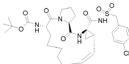
Compound 2119
