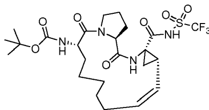
Compound 2107
