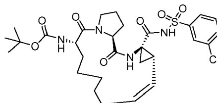
Compound 2110
