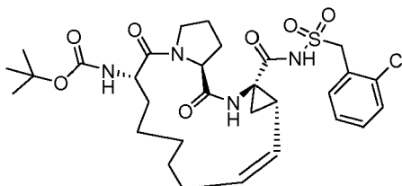
Compound 2117
