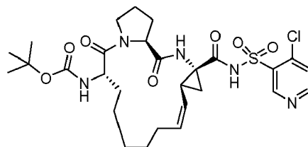
Compound 2128
