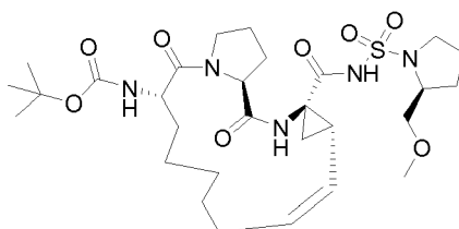
Compound 2252
