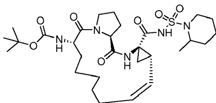
Compound 2225
