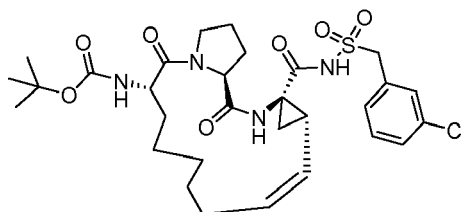
Compound 2118
