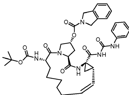
Compound 704
