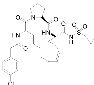
Compound 2143
