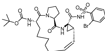
Compound 2111
