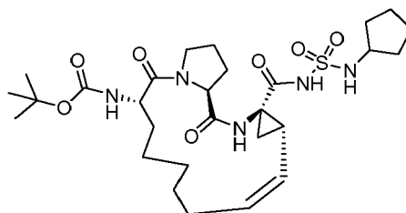
Compound 2215
