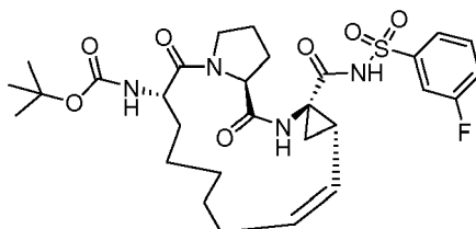
Compound 2113
