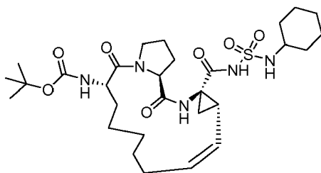
Compound 2205
