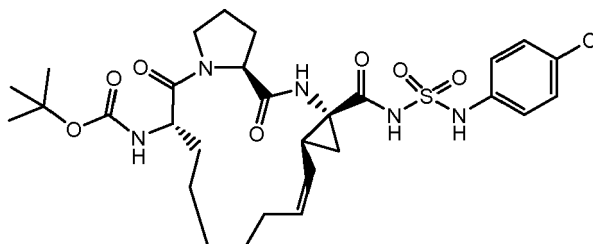
Compound 2247
