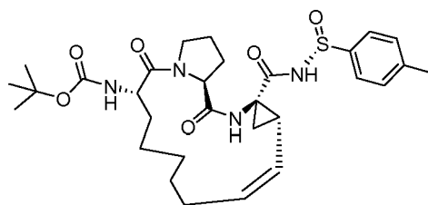
Compound 2403
