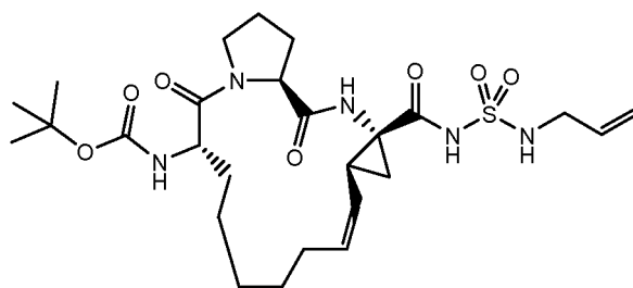
Compound 2238
