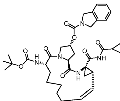
Compound 701
