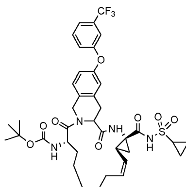
Compound 2008
