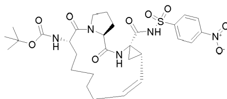
Compound 2102
