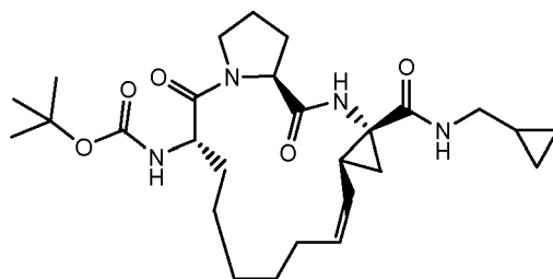
Compound A
