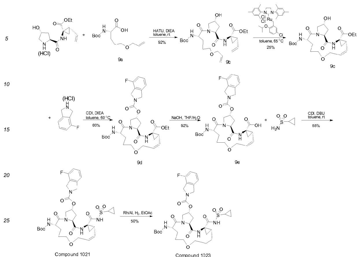
Scheme 9
