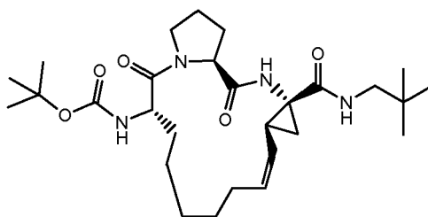
Compound 2315
