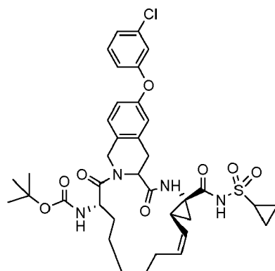
Compound 2007
