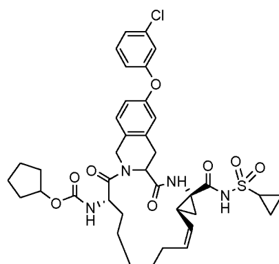
Compound AR00320573
