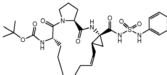
Compound 2246
