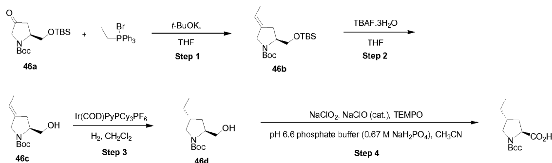
Scheme 4a
