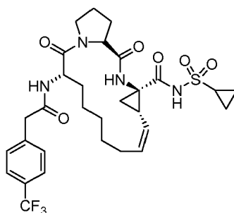
Compound 2142
