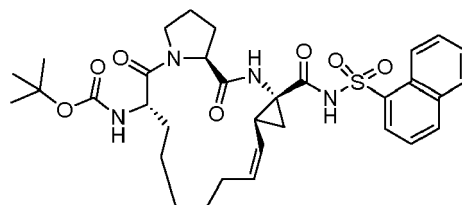
Compound 2148
