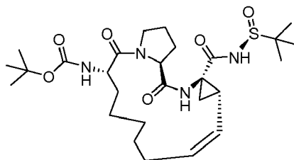
Compound 2401
