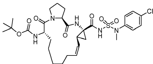
Compound 2226
