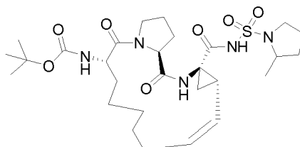
Compound 2250
