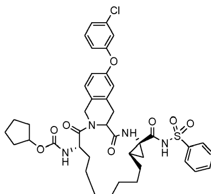
Compound 2010
