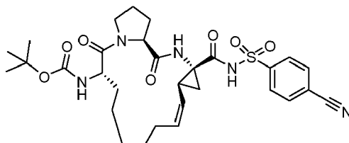
Compound 2134
