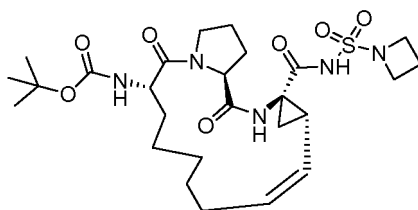
Compound 2206
