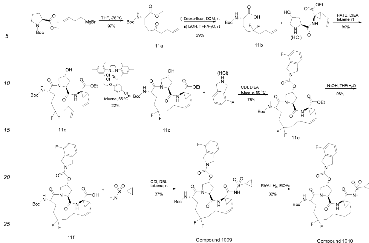
Scheme 11
