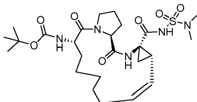
Compound 2202
