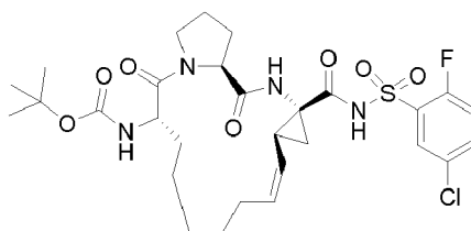
Compound 2150
