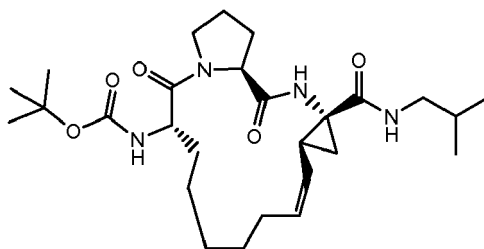
Compound 2314
