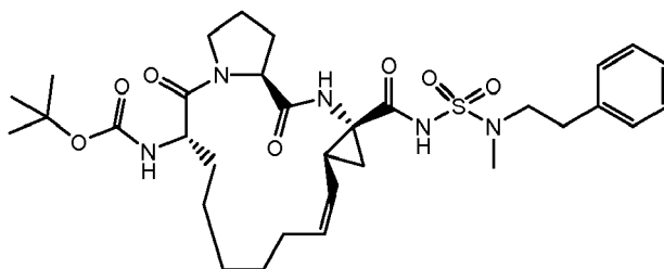
Compound 2248
