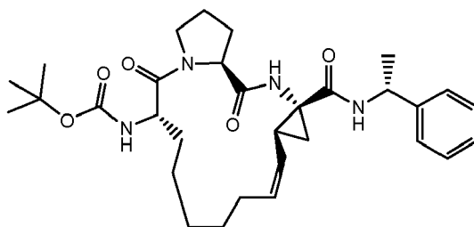
Compound 2311
