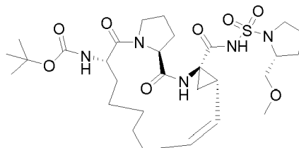
Compound 2251
