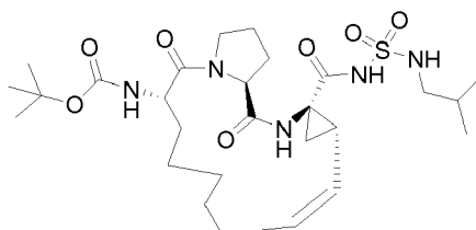
Compound 2218
