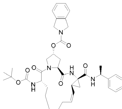
Compound 2502
