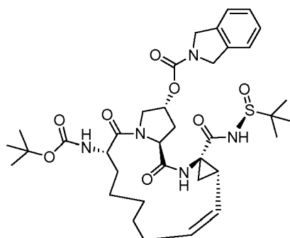
Compound 2601
