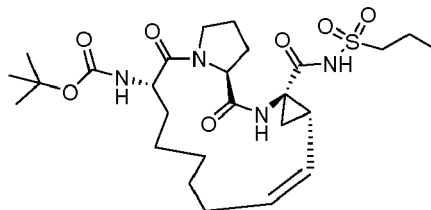
Compound 2105
