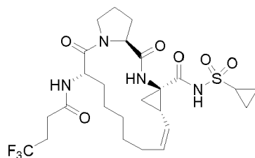
Compound 2139
