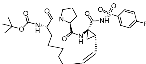
Compound 2114
