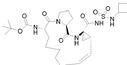
Compound 2214
