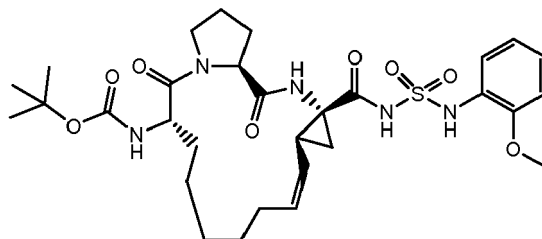
Compound 2236
