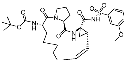
Compound 2116
