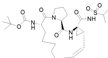
Compound 2104
