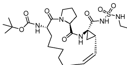
Compound 2216
