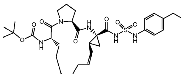
Compound 2242
