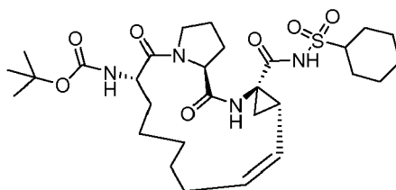
Compound 2121
