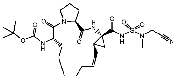
Compound 2249
