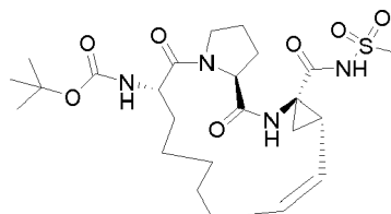
Compound 2103
