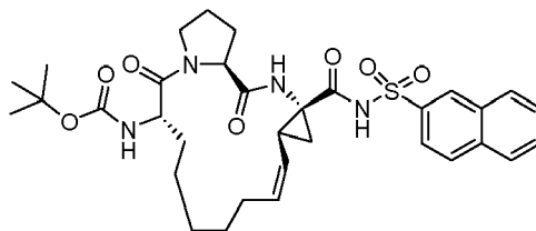
Compound 2130
