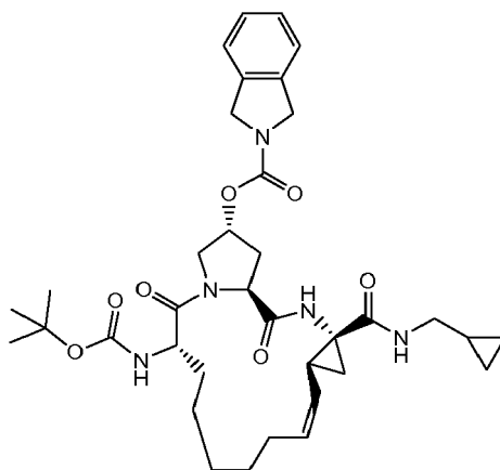
Compound 2501
