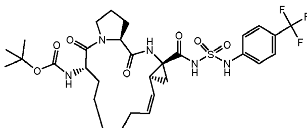
Compound 2235
