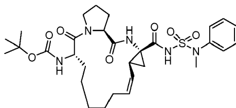
Compound 2227
