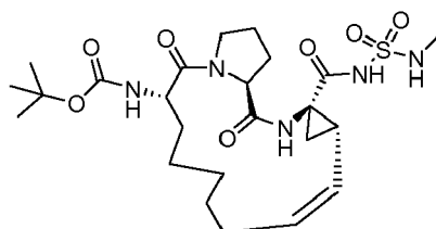
Compound 2213
