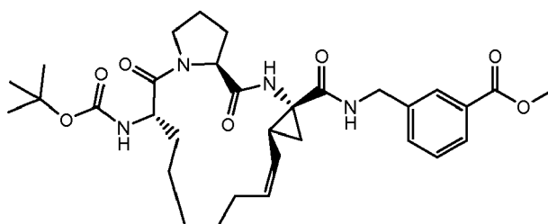
Compound 2321
