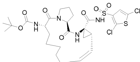
Compound 2126
