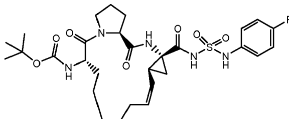
Compound 2237
