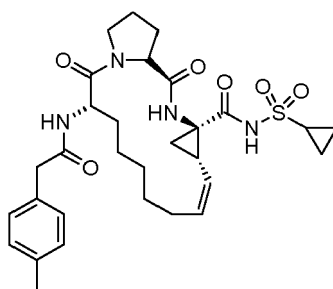
Compound 2140
