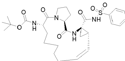
Compound 2101
