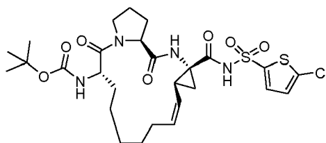
Compound 2132
