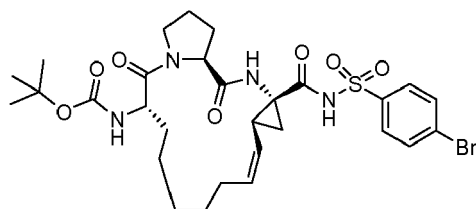
Compound 2131
