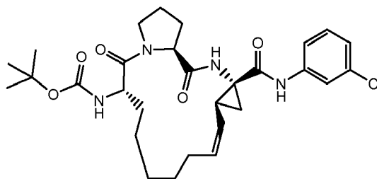
Compound 2317
