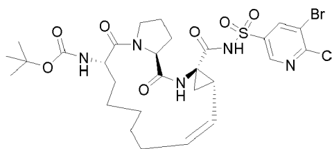
Compound 2154
