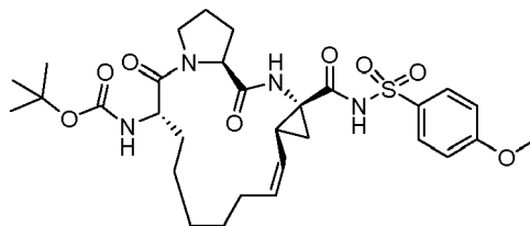
Compound 2133
