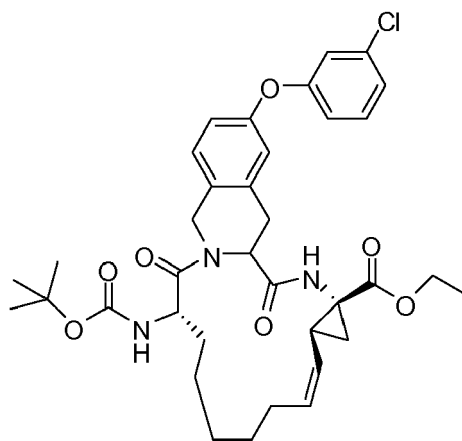
Compound 2006
