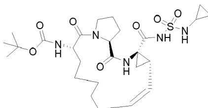
Compound 2201
