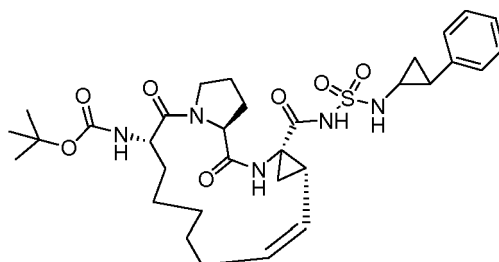
Compound 2224
