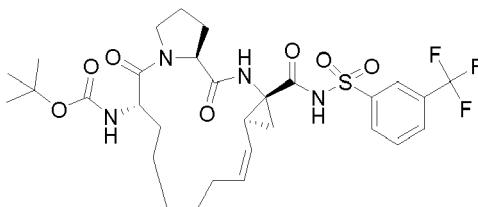
Compound 2149
