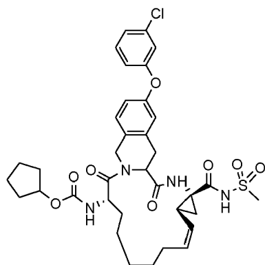
Compound 2003
