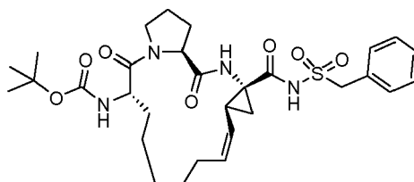
Compound 2135
