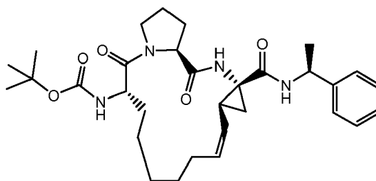
Compound 2301
