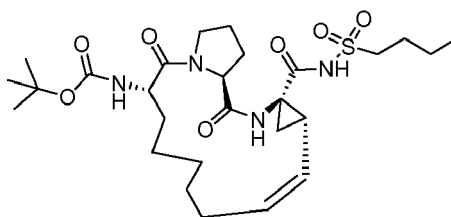
Compound 2106
