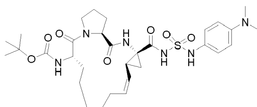
Compound 2231
