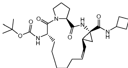
Compound 2303
