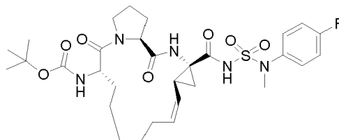
Compound 2229
