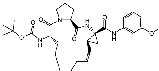
Compound 2312
