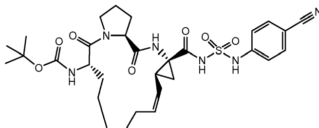
Compound 2241
