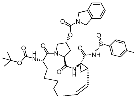
Compound 2603
