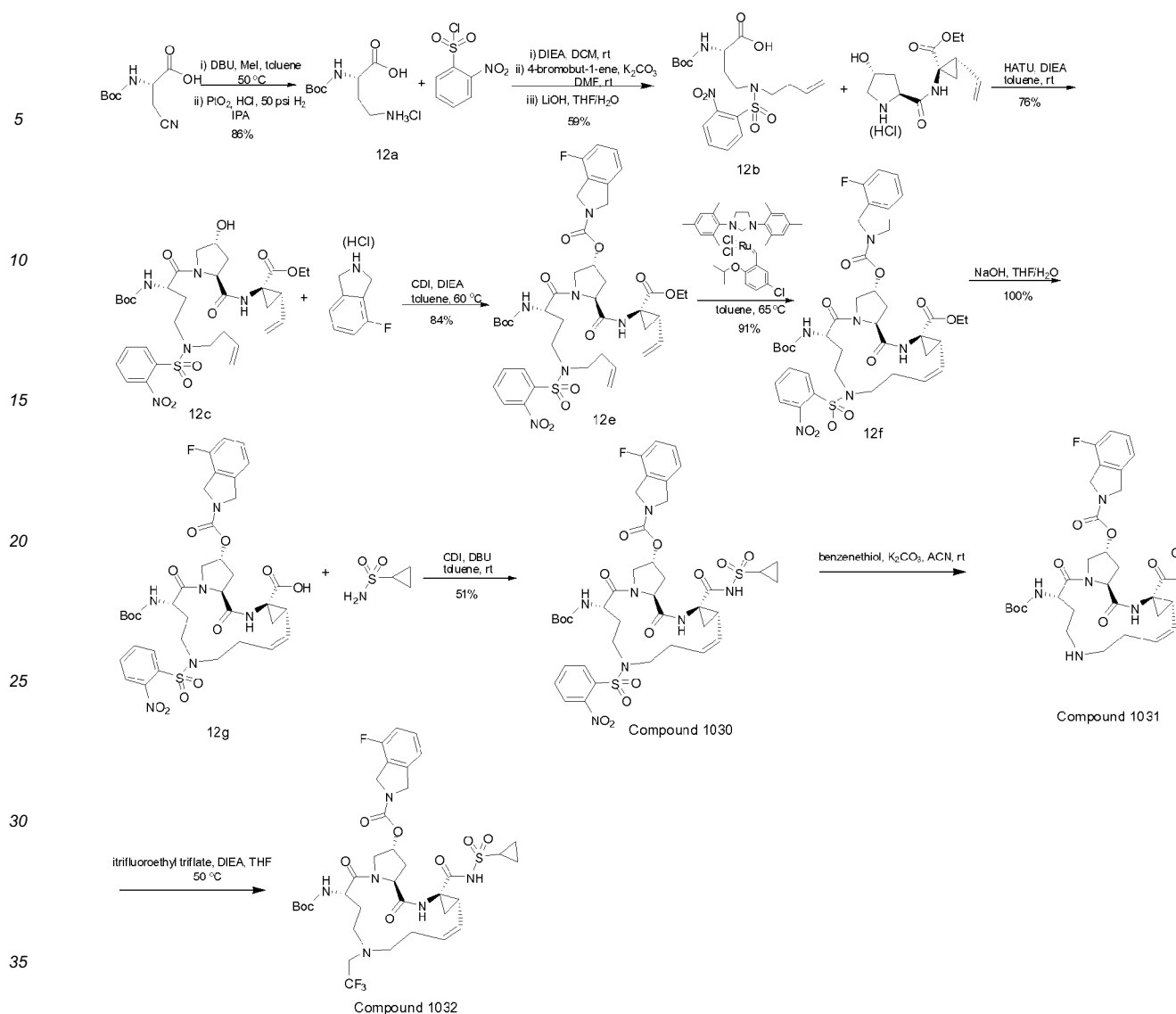
Scheme 12
