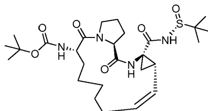
Compound 2404
