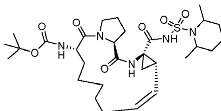
Compound 2223
