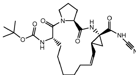
Compound 2306
