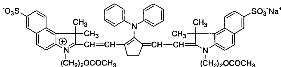
infrared absorber (8)
