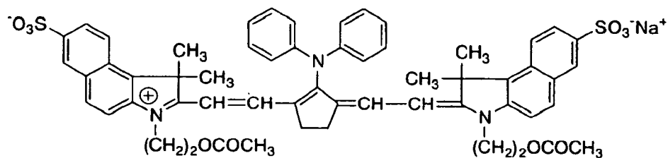
infrared absorber (8)
