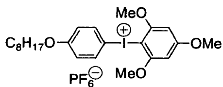
polymerization initiator (1)
