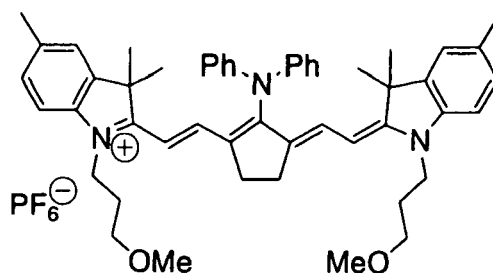
infrared absorber (1)
