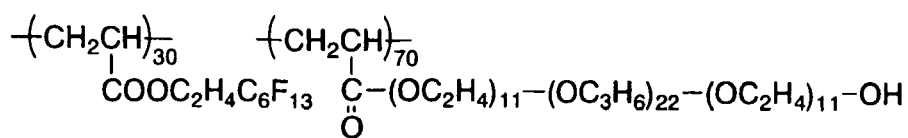
fluorosurfactant (1)
