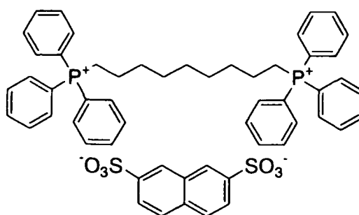
phosphonium compound (1)
