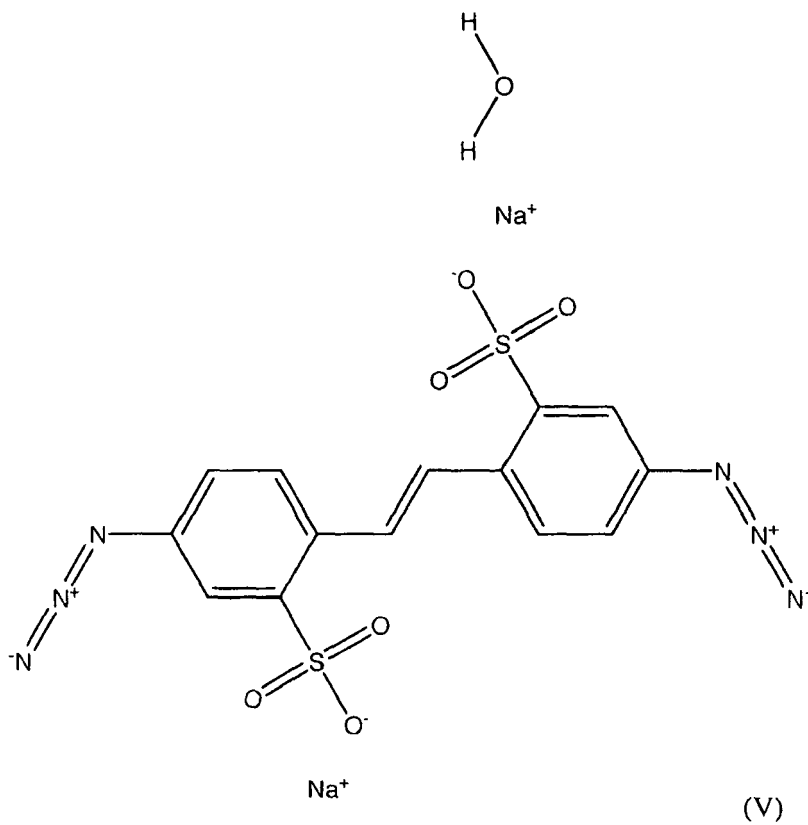
4,4'-Diazido-2,2'-stilbenedisulfonic acid disodium salt hydrate
