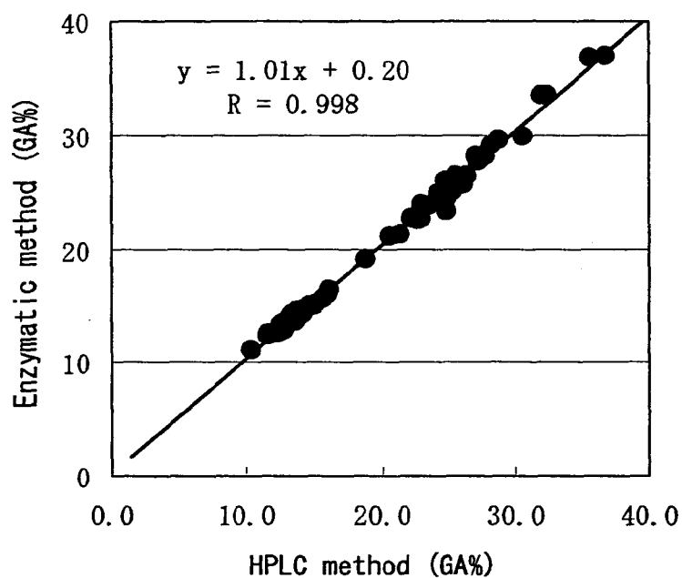
Fig. 10 Reaction curve for composition using second reagent containing protease
