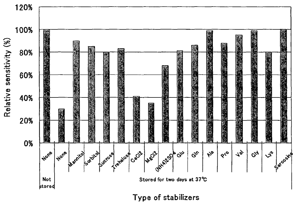
Fig. 6 Stabilization of glycated amino acid stabilizer
