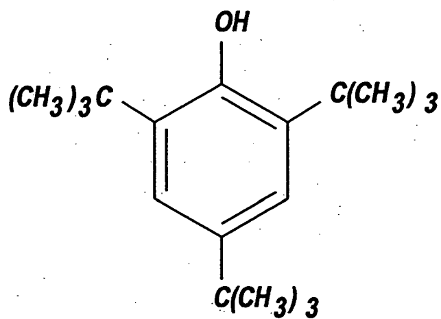
Butylated hydroxytoluene
