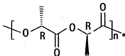
poly (D-lactide)
