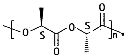
poly (L-lactide)
