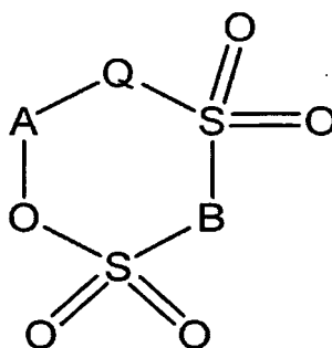
Chemical formula 2
