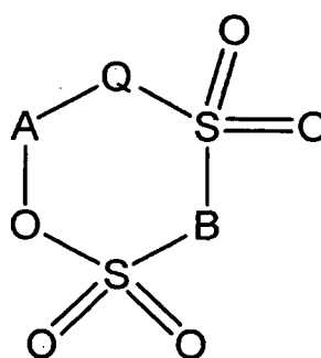
Chemical formula 2
