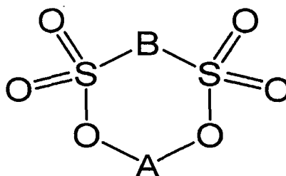
Chemical formula 1
