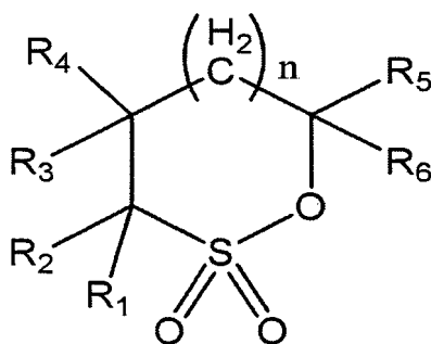
Chemical formula 3
