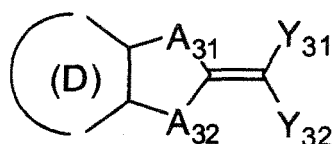
Formula (3)
