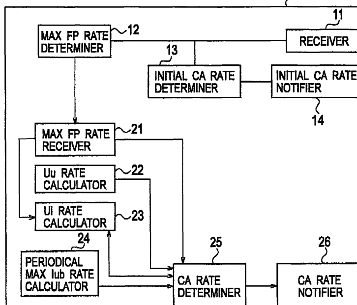
FIG. 4 RADIO BASE STATION BTS
