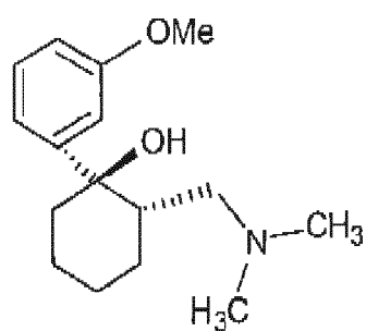
(R,S) trans
