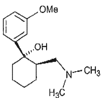
(S,R) trans
