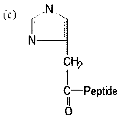
Imidazoacetyl (CA)-Exendin-4
