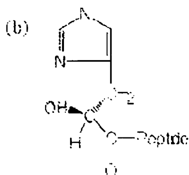
Beta-hydroxy-imidazopropyl (HY)-Exendin-4
