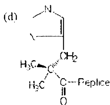
Dimethyl-histidyl (DM)-Exendin-4
