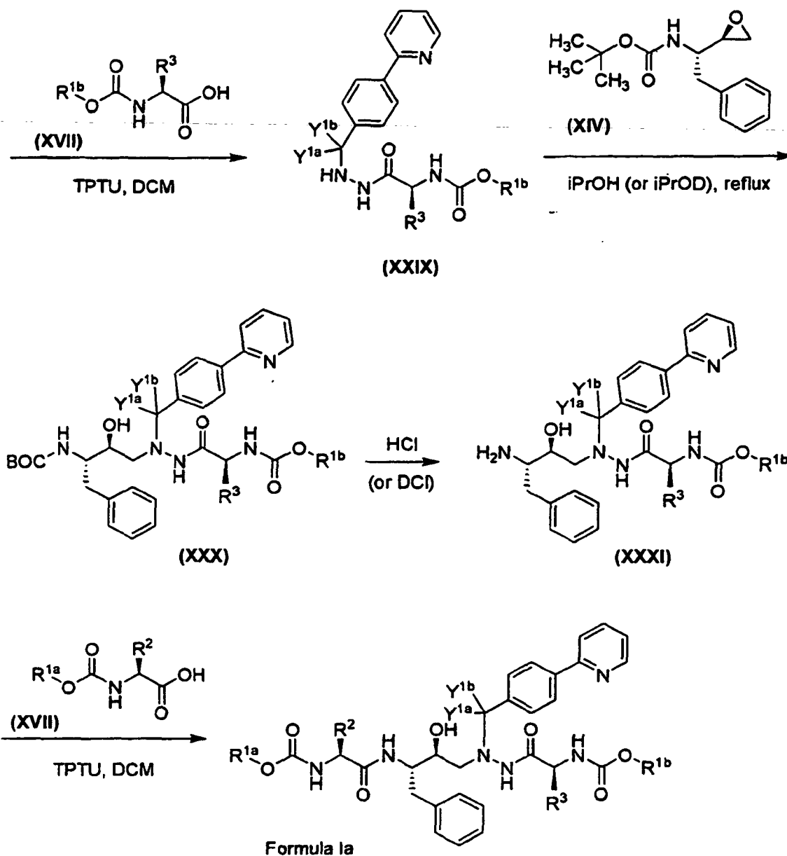
[0061] Scheme 1c. General Route for Incorporating Different R and Y Groups.
