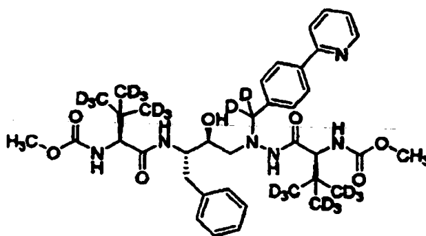
Compound 113
