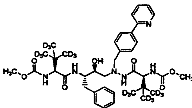
Compound 106
