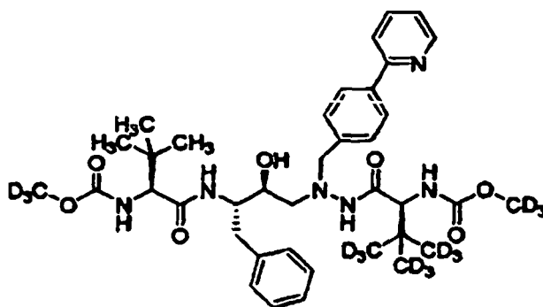
Compound 121
