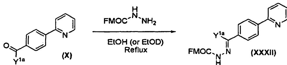
[0061] Scheme 1c. General Route for Incorporating Different R and Y Groups.
