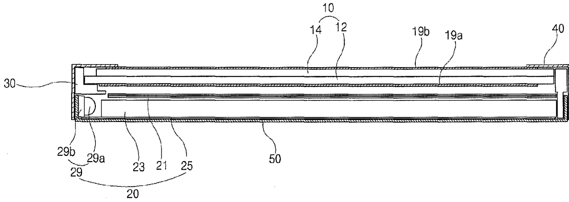
FIG. 1 RELATED ART
