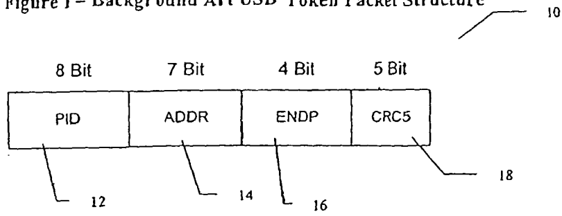
Figure 1 – Background Art USB Token Packet Structure
