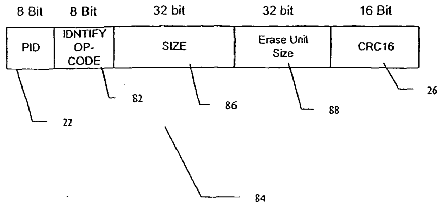
Fig 8 – Flash Identification Replay Packet
