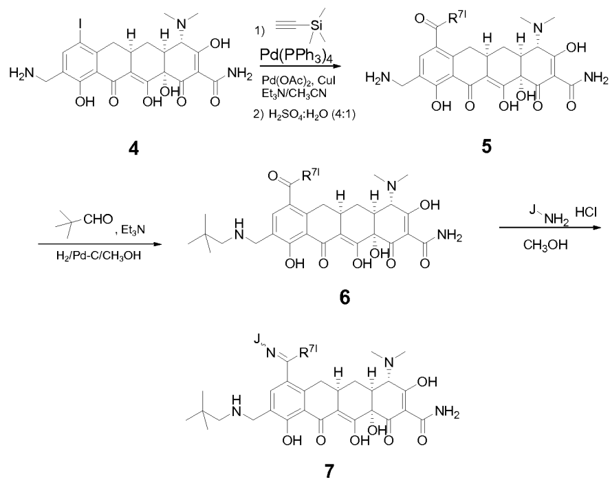
Scheme 2
