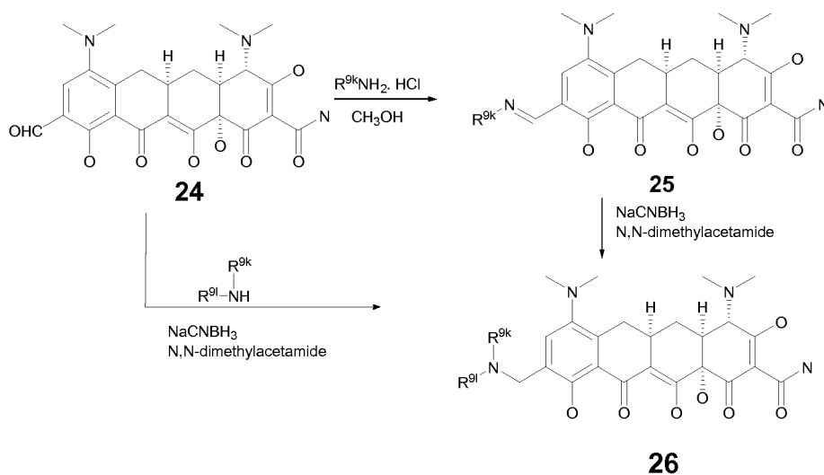
Scheme 11
