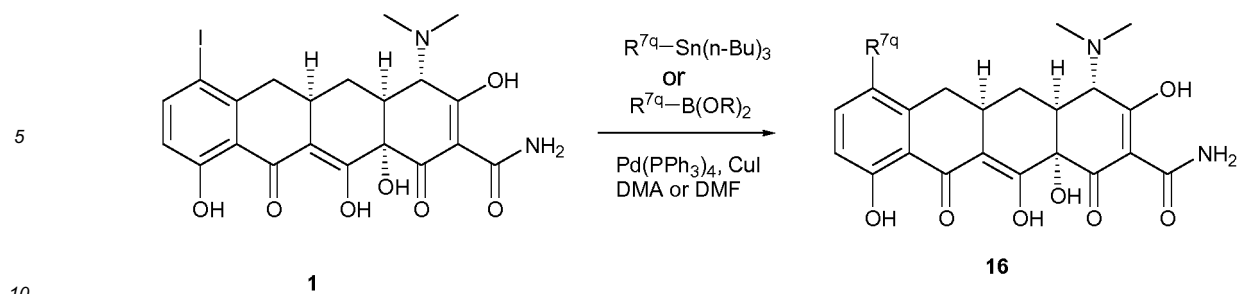
Scheme 6
