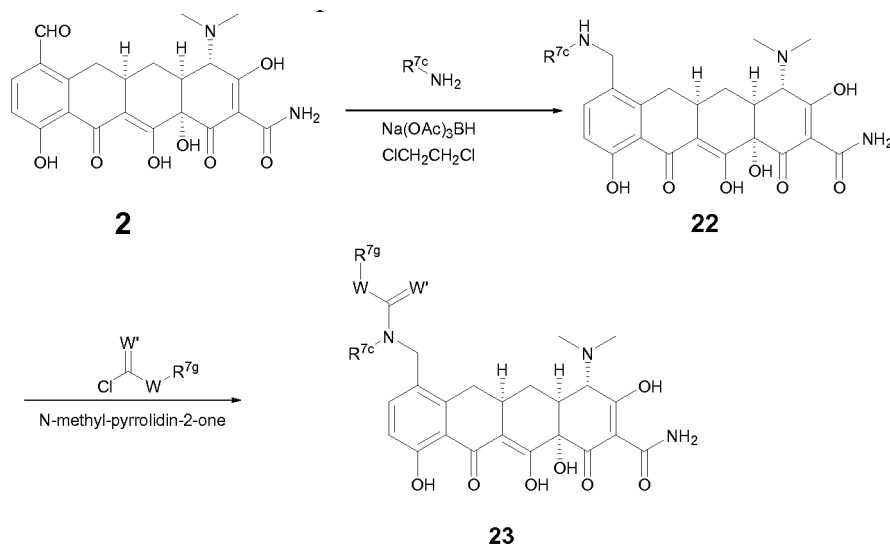
Scheme 10
