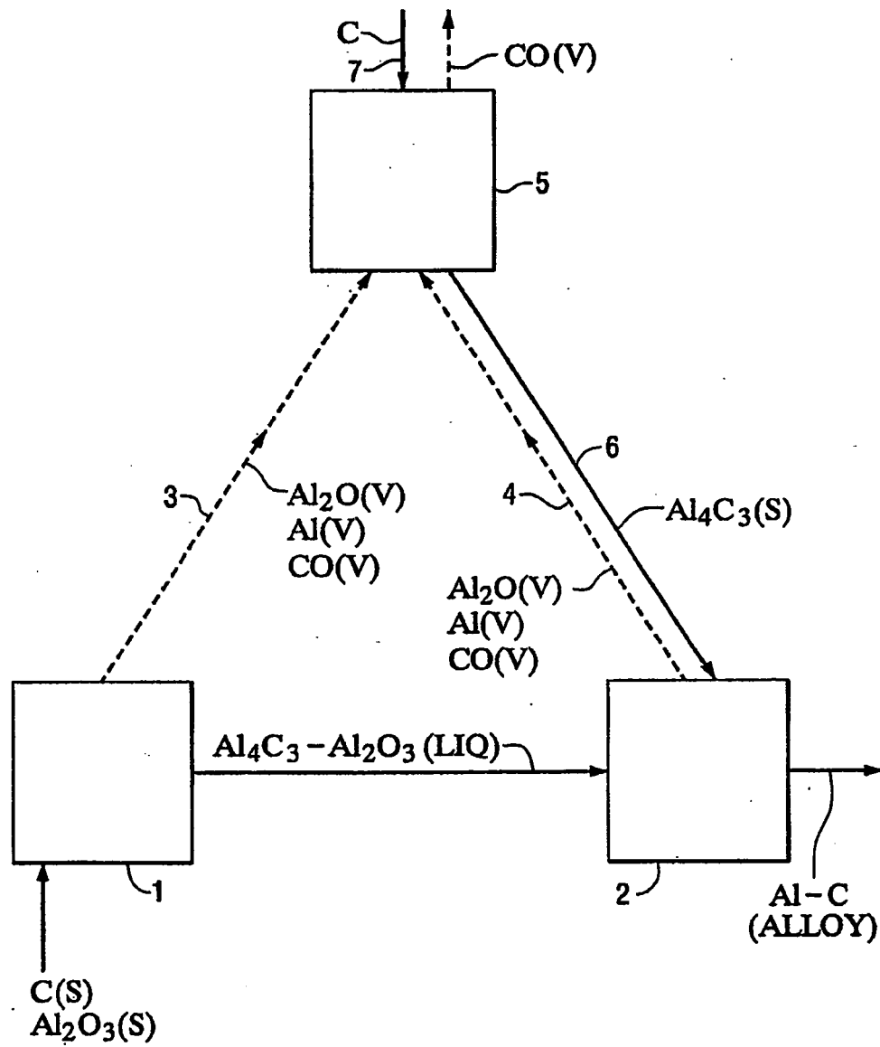
FIG. 1 PRIOR ART
