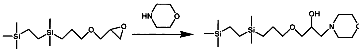
Figure 12. Reaction Sequence for Preparation of Silane 12.
