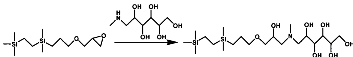
Figure 24. Reaction Sequence for Preparation of Silane 24.
