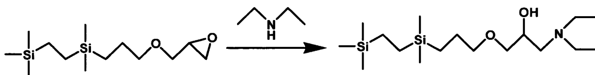
Figure 19. Reaction Sequence for Preparation of Silane 19.
