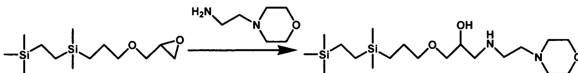
Figure 17. Reaction Sequence for Preparation of Silane 17.
