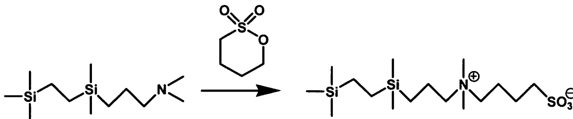
Figure 3. Reaction Sequence for Preparation of Silane 3.
