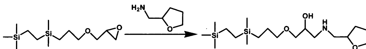
Figure 18. Reaction Sequence for Preparation of Silane 18.
