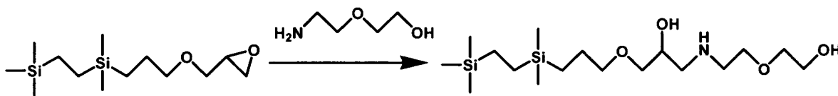
Figure 10. Reaction Sequence for Preparation of Silane 10.
