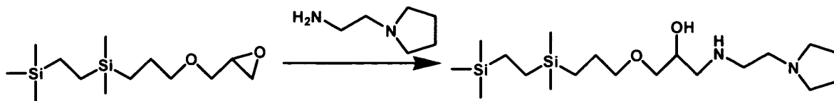
Figure 15. Reaction Sequence for Preparation of Silane 15.
