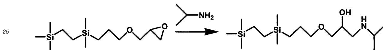
Figure 22. Reaction Sequence for Preparation of Silane 22.
