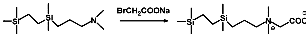
Figure 4. Reaction Sequence for Preparation of Silane 4.
