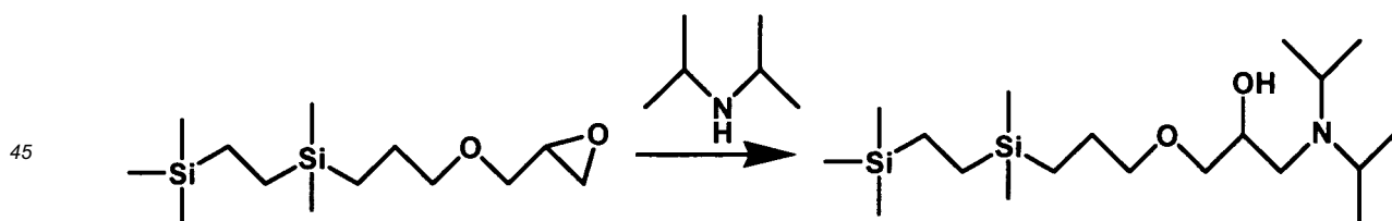
Figure 23. Reaction Sequence for Preparation of Silane 23.
