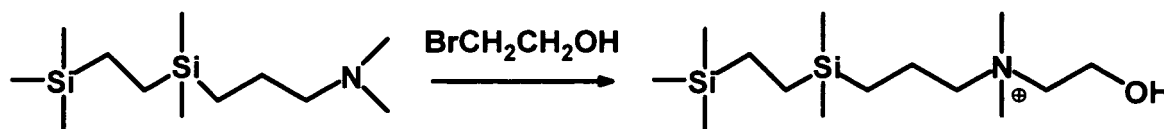
Figure 5. Reaction Sequence for Preparation of Silane 5.
