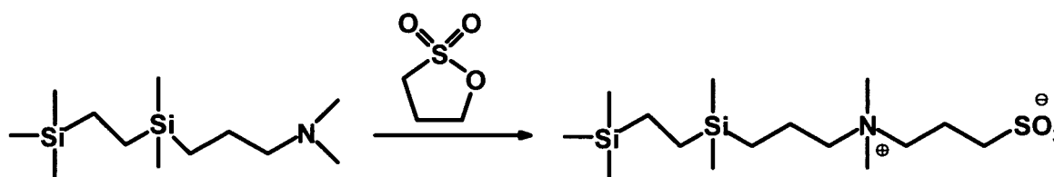
Figure 2. Reaction Sequence for Preparation of Silane 2.
