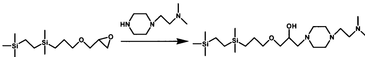
Figure 14. Reaction Sequence for Preparation of Silane 14.
