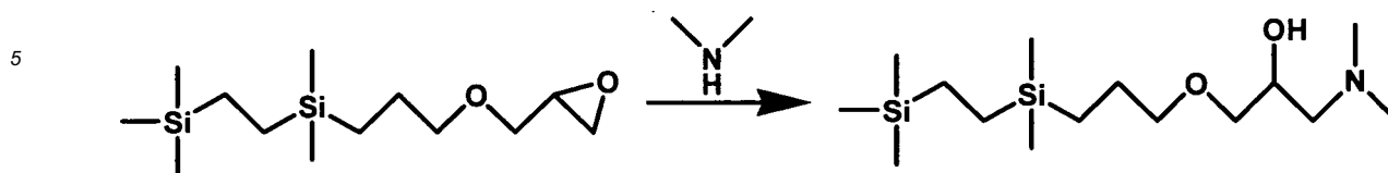
Figure 21. Reaction Sequence for Preparation of Silane 21.
