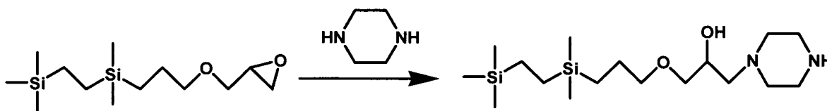
Figure 13. Reaction Sequence for Preparation of Silane 13.
