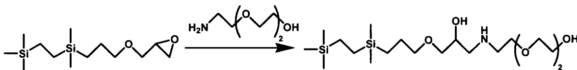
Figure 11. Reaction Sequence for Preparation of Silane 11.
