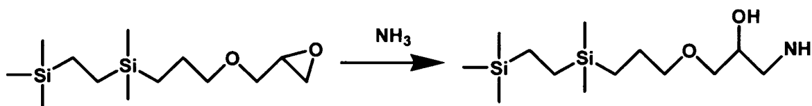
Figure 20. Reaction Sequence for Preparation of Silane 20.
