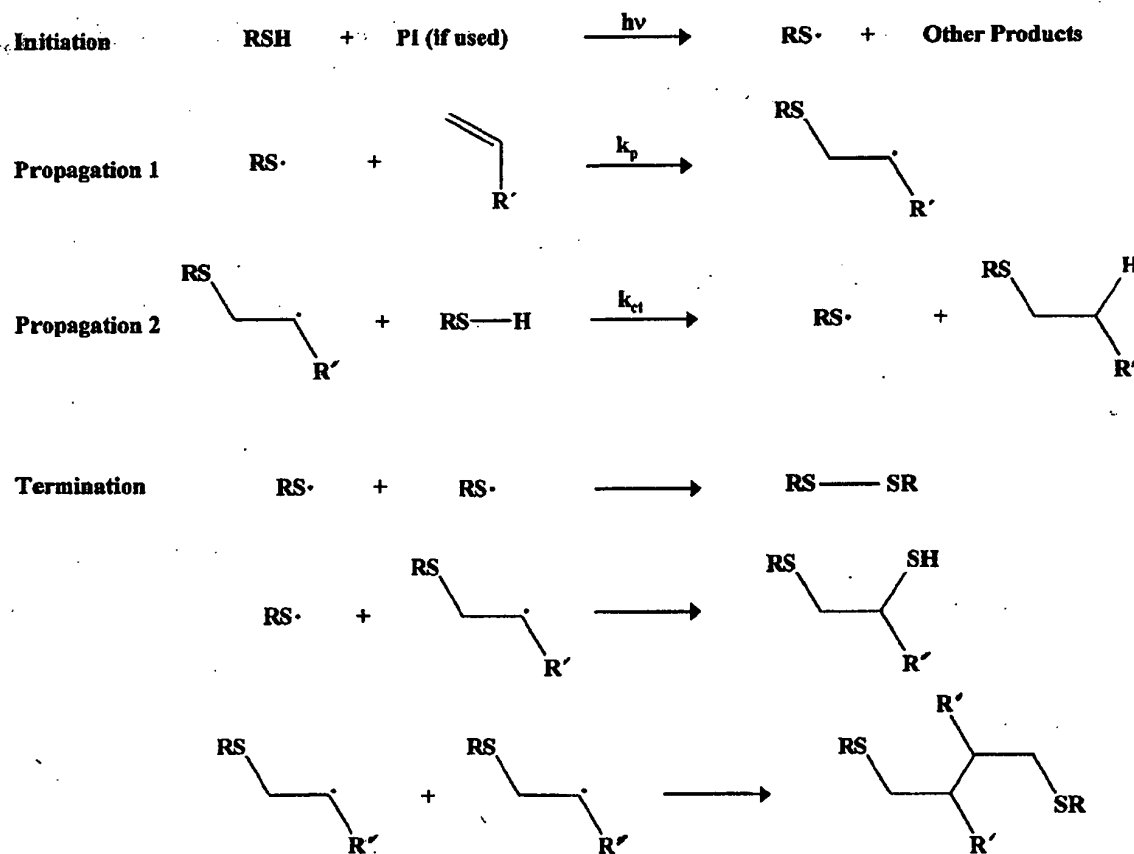
Scheme 1. General thiol-ene photopolymerization process.
