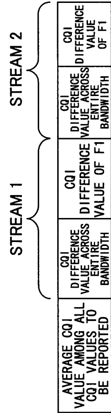
FIG.5C CQI BITS CONFIGURATION IN CQI TTI (CASE 2)
