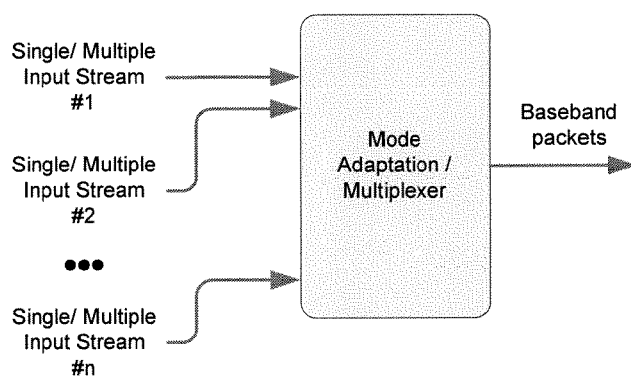
Figure 25: Mode adaptation for DVB-C2, supporting single and multiple input streams (TS or GS)
