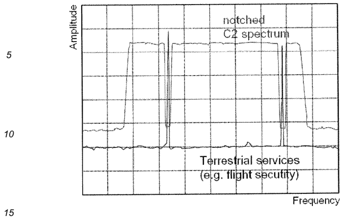
Figure 36: Example of notched C2 OFDM spectrum (red curve) and terrestrial services (e.g. flight security service, blue curve), sharing the same frequency range
