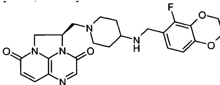
(a) 5-Fluoro-2,3-dihydro-1,4-benzodioxin
