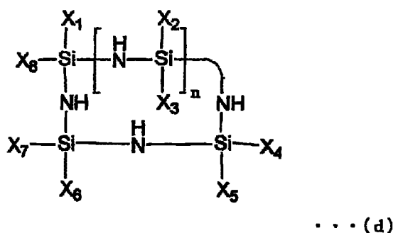
[Chemical 4]
