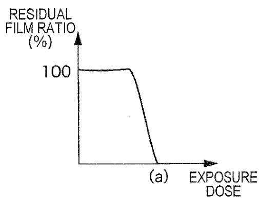
EXPOSURE DOSE-RESIDUAL FILM CURVE WHEN POSITIVE TONE DEVELOPER IS USED
