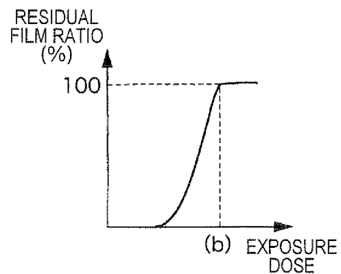
EXPOSURE DOSE-RESIDUAL FILM CURVE WHEN NEGATIVE TONE DEVELOPER IS USED
