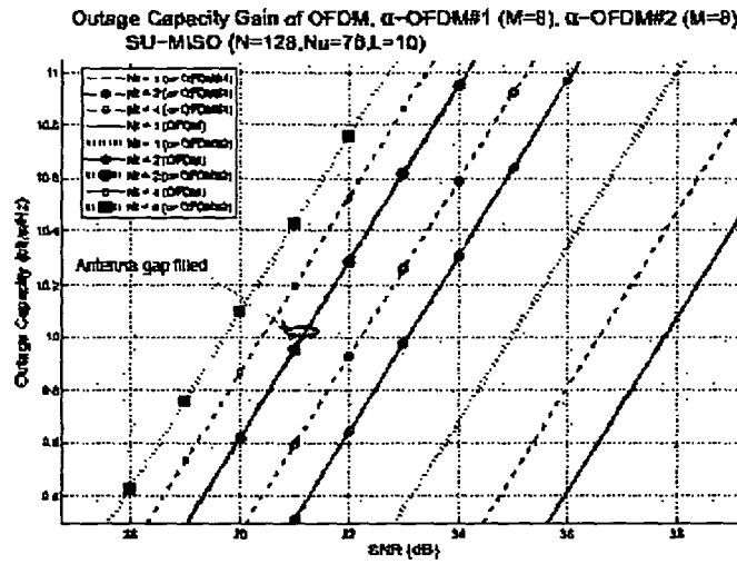
Fig. 7. Outage Capacity gain for \alpha -OFDM MISO
