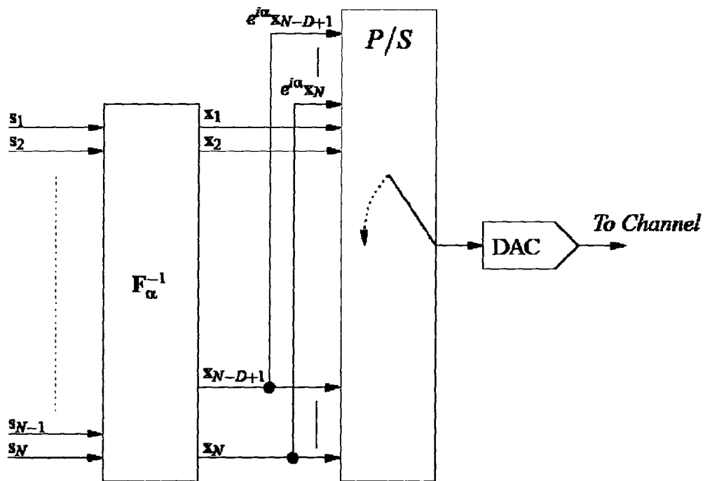
Fig. 1. \alpha -OFDM Transmission Scheme
