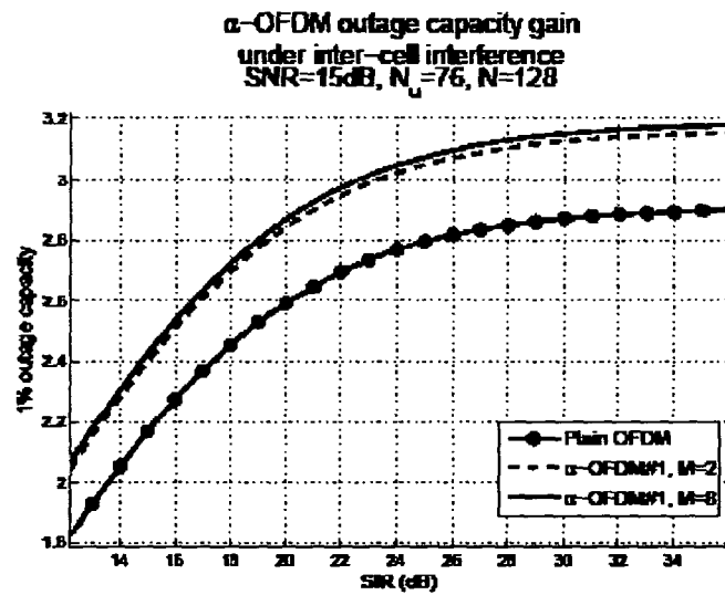
Fig. 6. \alpha -OFDM#1 with Inter-Cell Interference
