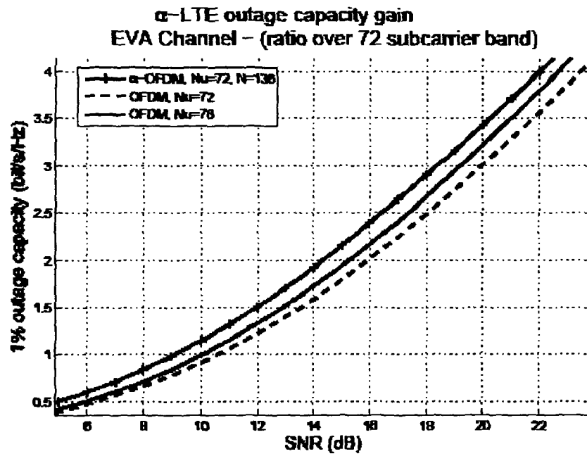
Fig. 9. LTE & \alpha -LTE outage capacity
