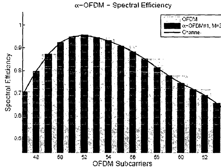
Fig. 3. Spectral efficiency of \alpha -OFDM
