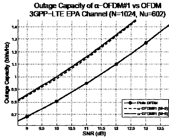
Fig. 4. \alpha -OFDM#1 Outage Capacity in 3GPP-LTE EPA
