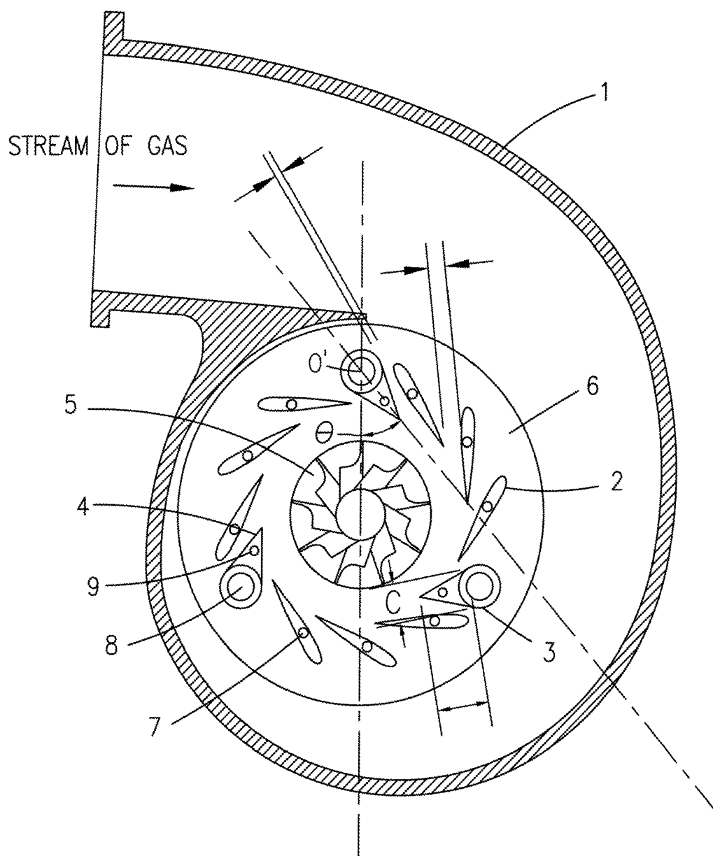
Fig. 2 Prior Art
