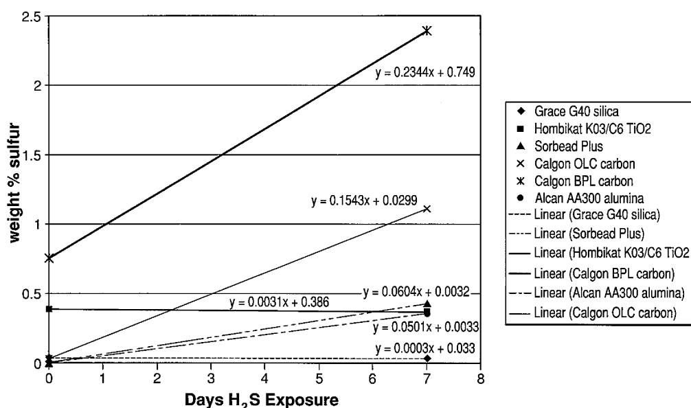
FIG. 1 Sulfur Deposition Rate
