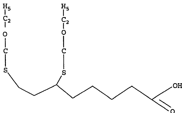
Diethoxycarbonylated Lipoic Acid
