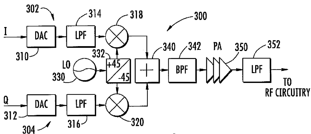
FIG. 6 (PRIOR ART)
