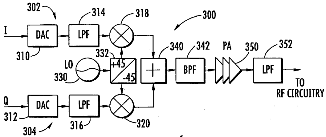
FIG. 6 (PRIOR ART)
