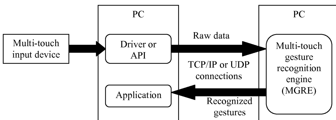
Figure 2: Example of distributed architecture
