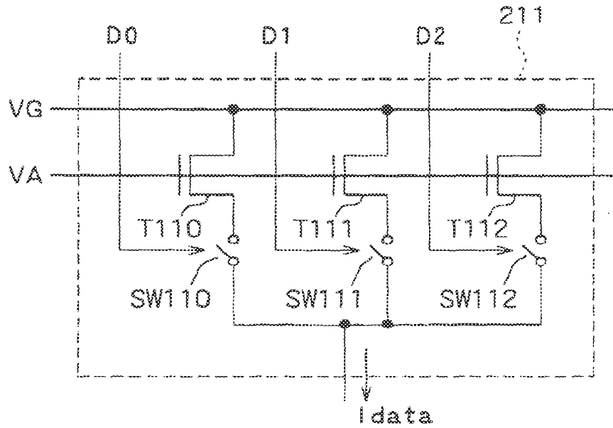
FIG. 6 (PRIOR ART)
