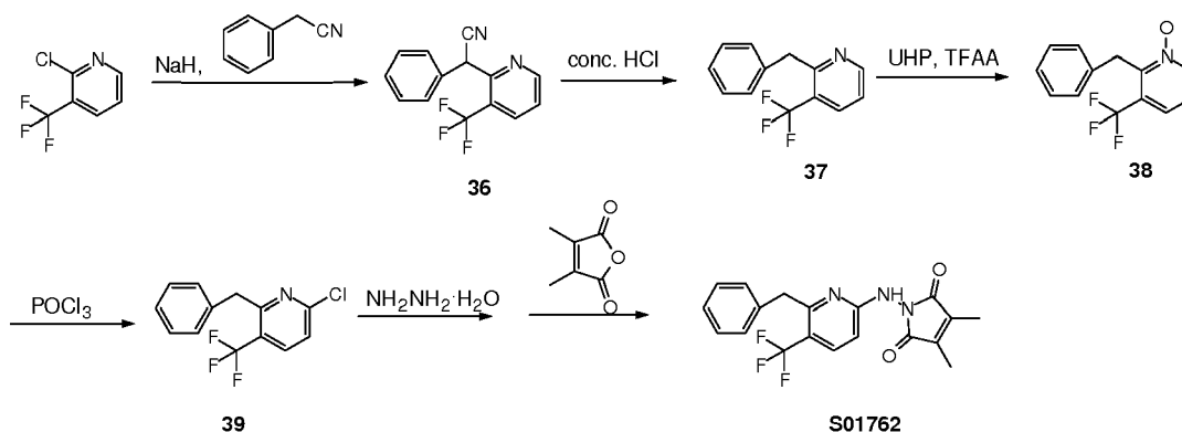
Scheme 20
