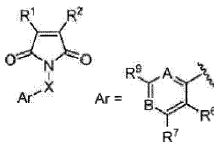
Structure (II)
