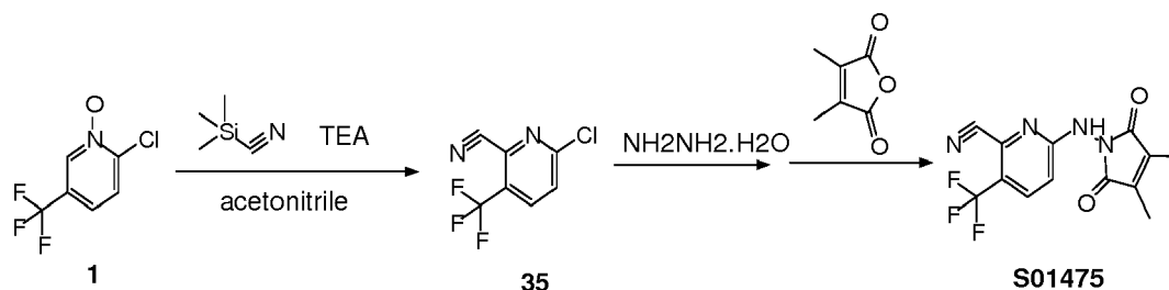
Scheme 19
