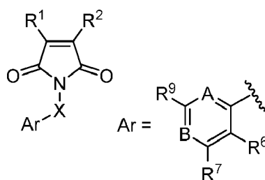
Structure (II)
