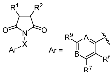
Structure (II)
