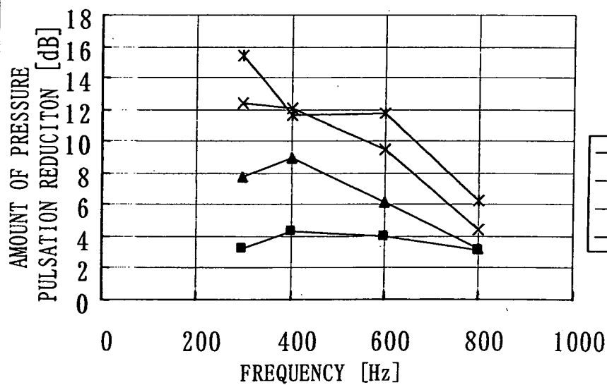
(2) PRESSURE PULSATION REDUCITON OF AIR JET SUCTION
