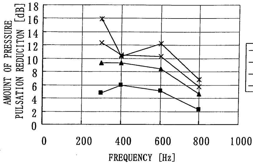
(1) PRESSURE PULSATION REDUCITON OF AIR JET BLOW
