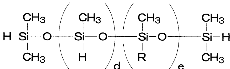
(Structural Formula 3)
