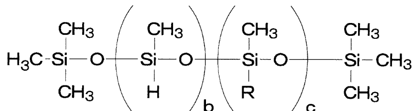
(Structural Formula 2)
