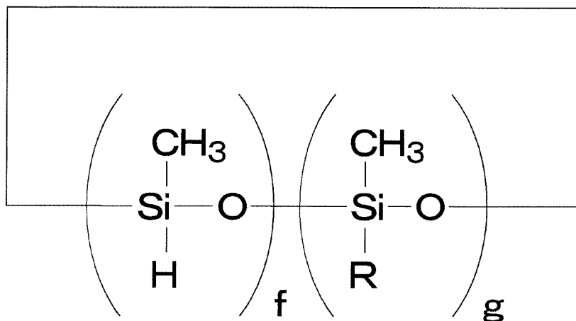
(Structural Formula 4)
