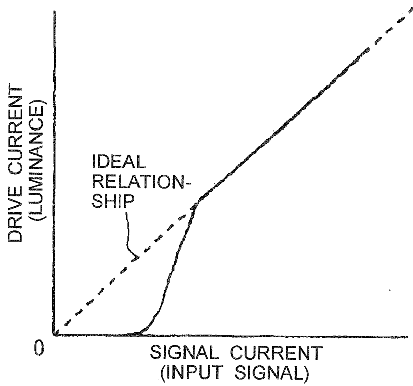
FIG. 3 (BACKGROUND ART)
