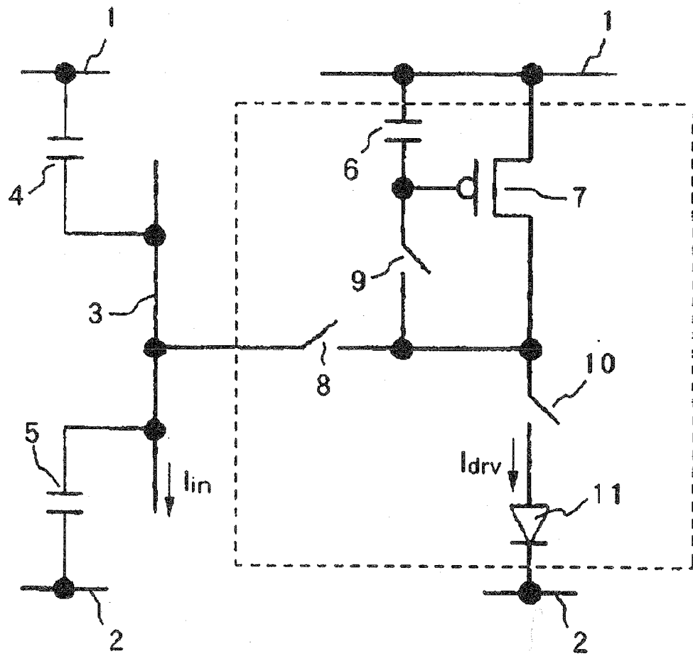
FIG. 1 (BACKGROUND ART)
