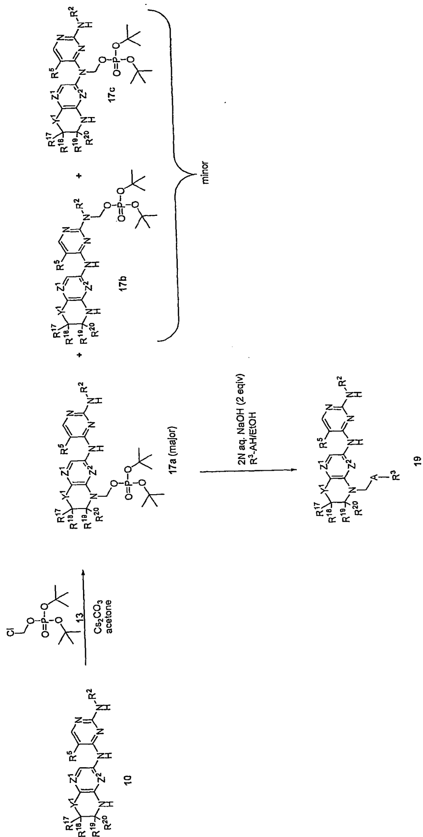
Scheme II
