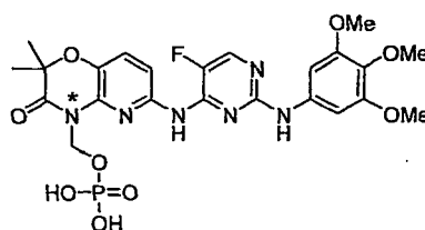
Compound 4
