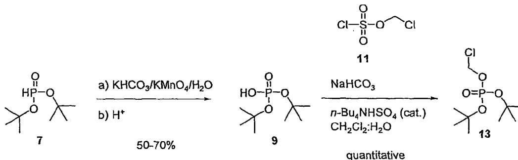
Scheme (III)
