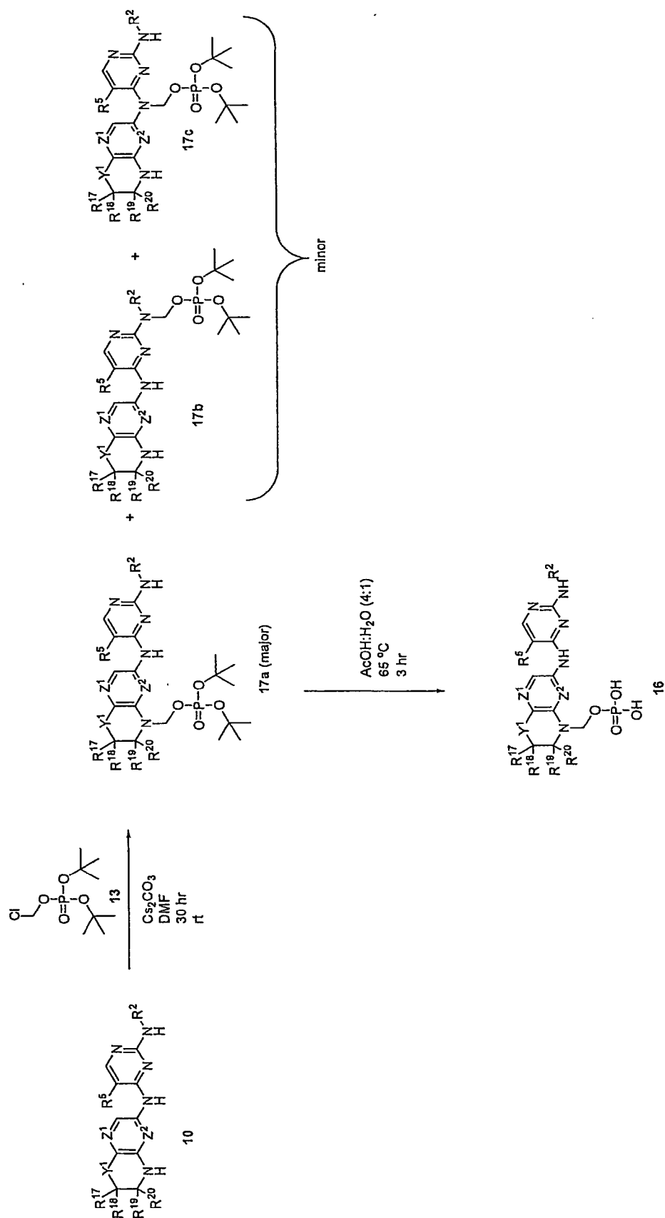
Scheme (V)
